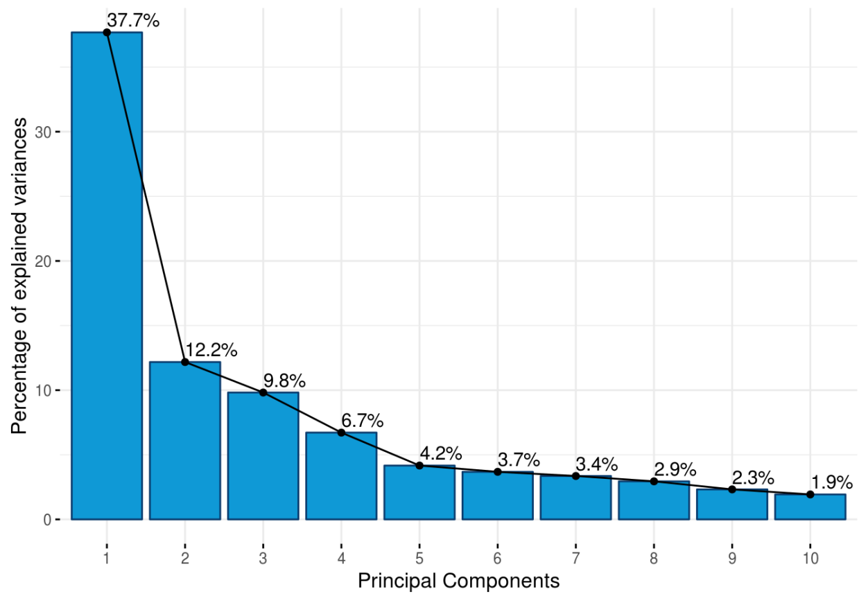
Supplemental Figure A1. Scree plot of explained variance by principal component from principal component analysis.
