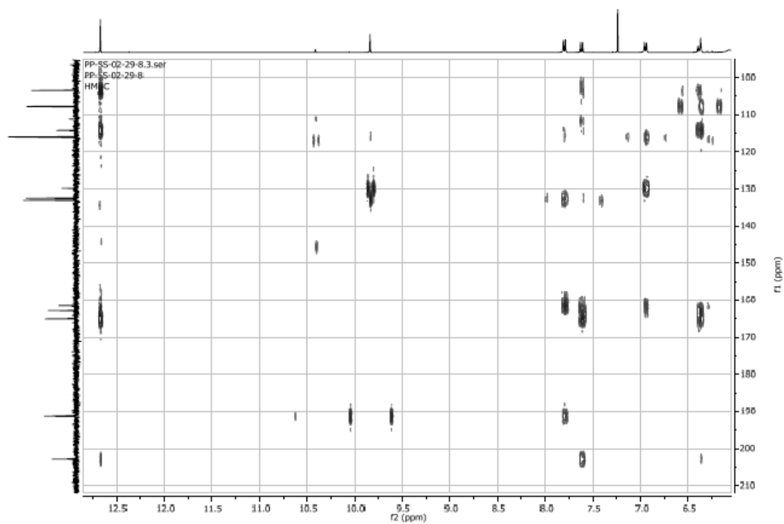
Figure S10: HMBC spectrum of Compound 1
