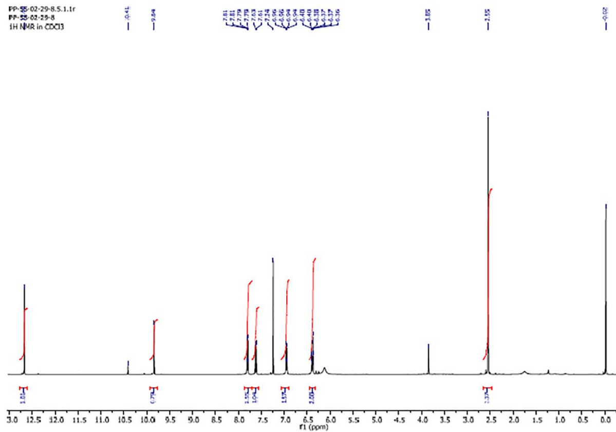
Figure S3: 1 H NMR of Compound 1
