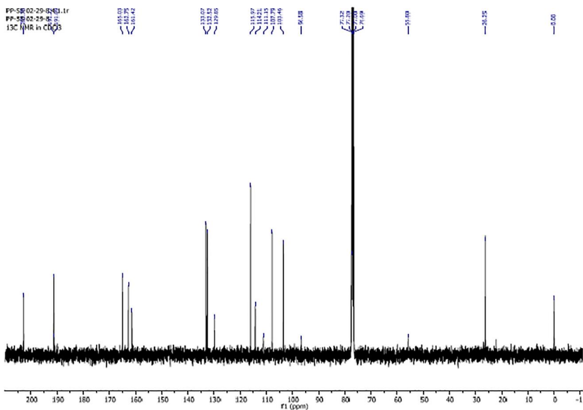
Figure S5: 13 C NMR of Compound 1
