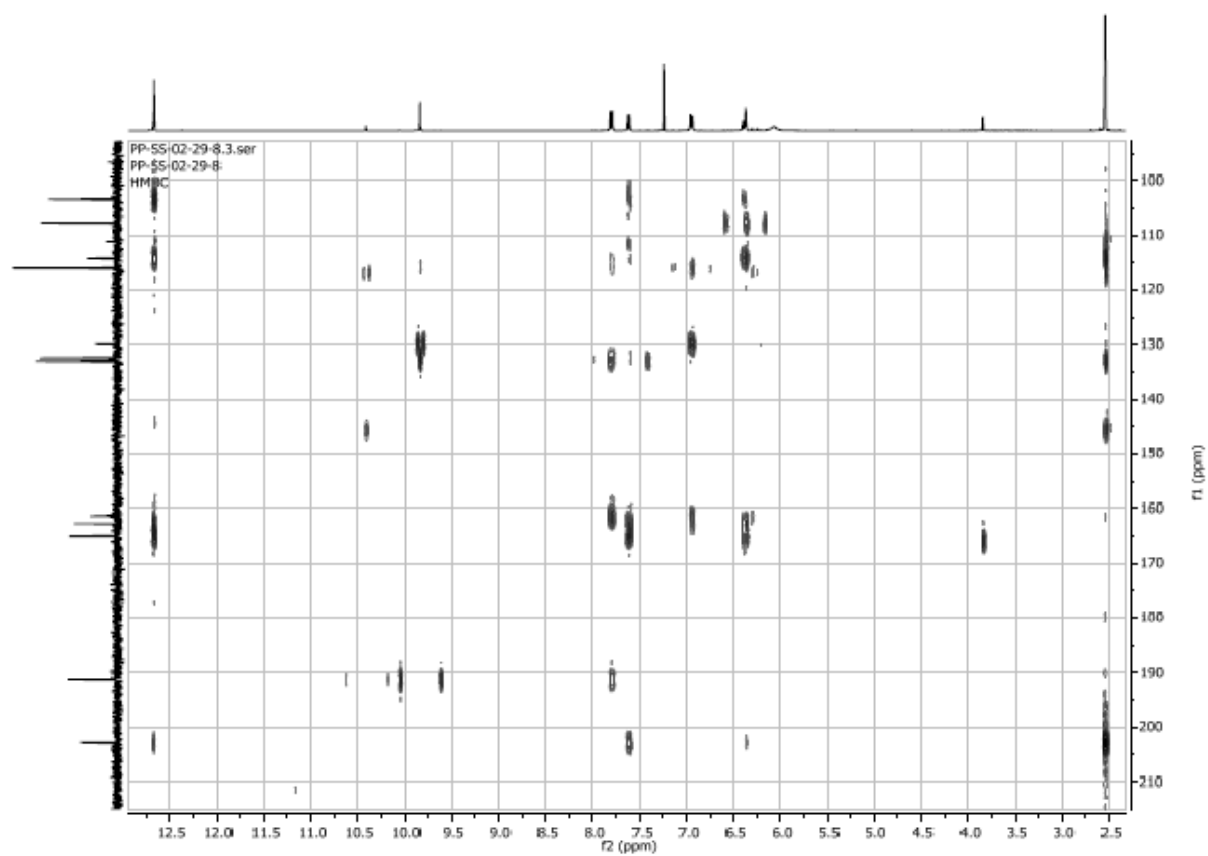
Figure S9: HMBC spectrum of Compound 1
