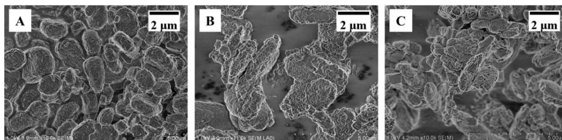
Figure S1. SEM images of EU-1 zeolites: A, EU-1-0; B, EU-1-1; C, EU-1-2
