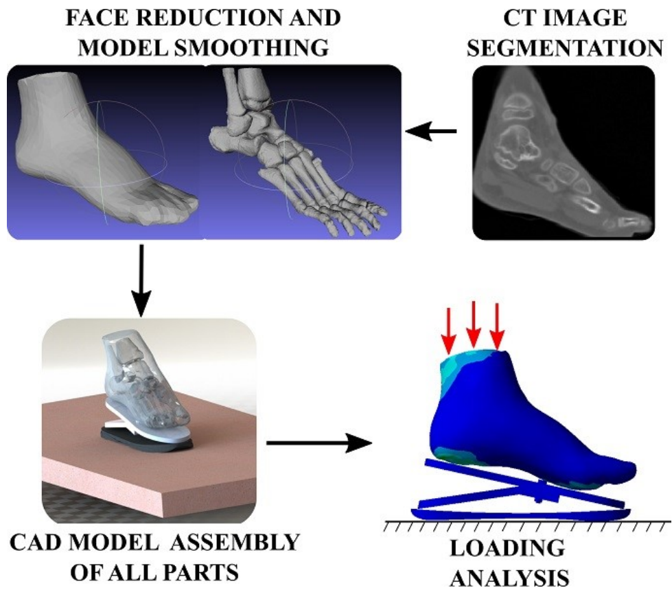
Figure A2 - The workflow adopted in the finite element analysis.
