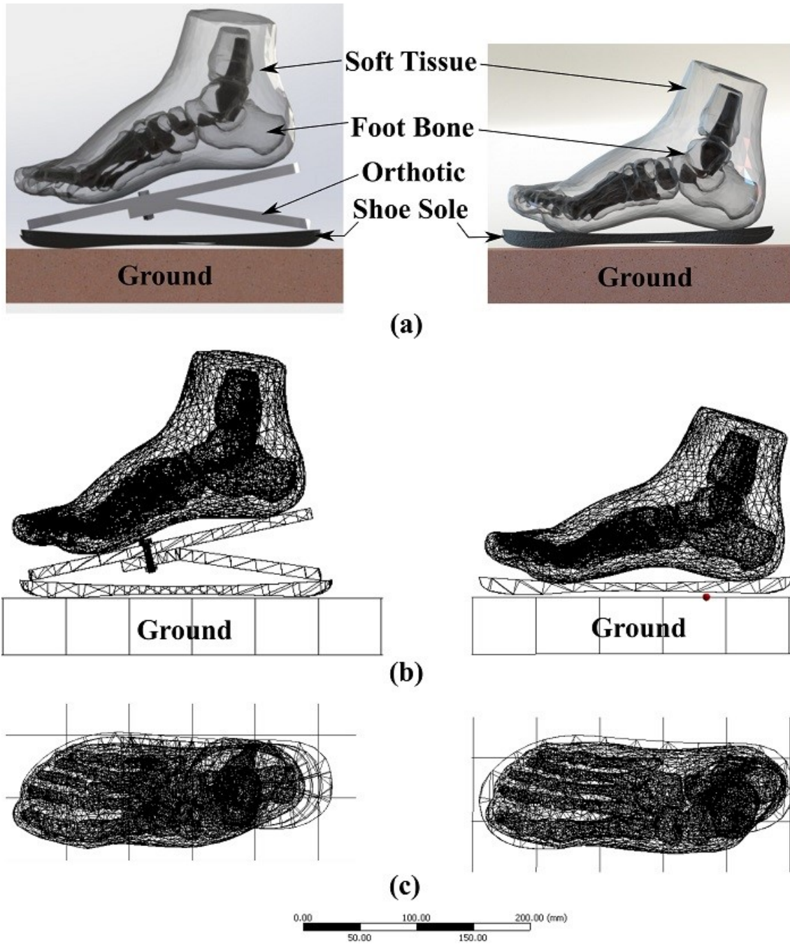
Figure A3 - (a) The foot bone and tissue assembly with and without orthotic, (b) side view of the meshed assembly, and (c) top view of the meshed assembly.
