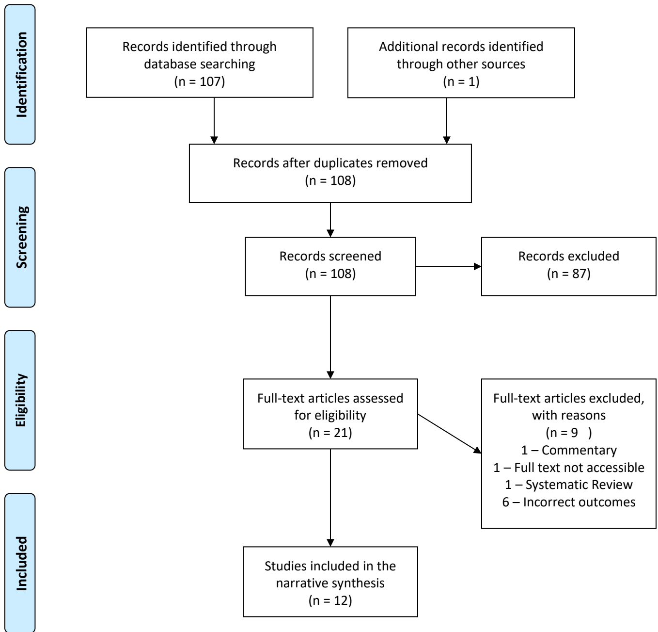
Figure S1: PRISMA Flow Diagram of the Literature Review on the Incidence of Stapler Malfunction
