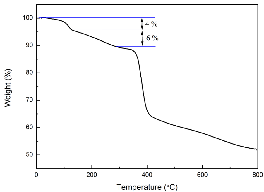
Figure S2 TG curve of compound 1
