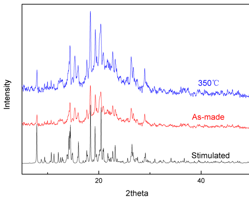
Figure S1 PXRD curve of compound 1
