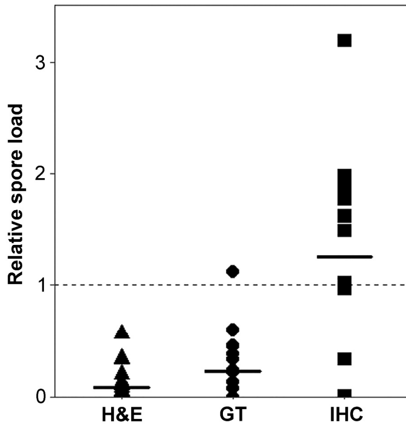
Supplementary Figure 1. Relative spore load detected with hematoxylin and eosin (H&E), Gram–Twort (GT), and immunohistochemistry (IHC) expressed as a ratio to calcofluor white (dashed line). The medians of the relative spore load detected with H&E, GT, and IHC are indicated by solid horizontal lines.
