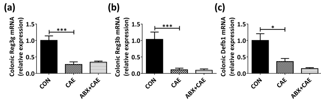
Figure S1. The chemical barrier-associated markers. Levels of colonic chemical barrier markers Reg3g (a), Reg3b (b) and Defb1 (c) were determined by qPCR. The results are shown as mean \pm SD, n \geq 3 . * p < 0.05 , ** p < 0.01 and *** p < 0.001 by one-way ANOVA followed by Dunnett's test.
