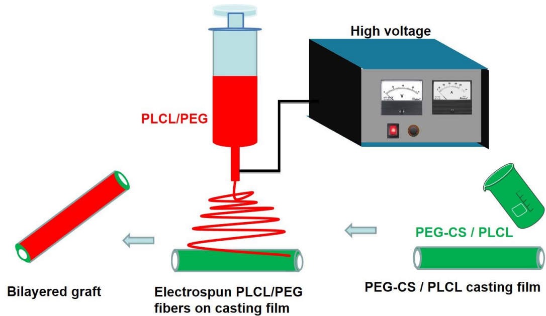
Figure.1 Schematic diagram of fabrication bilayered small-diameter vascular graft.
