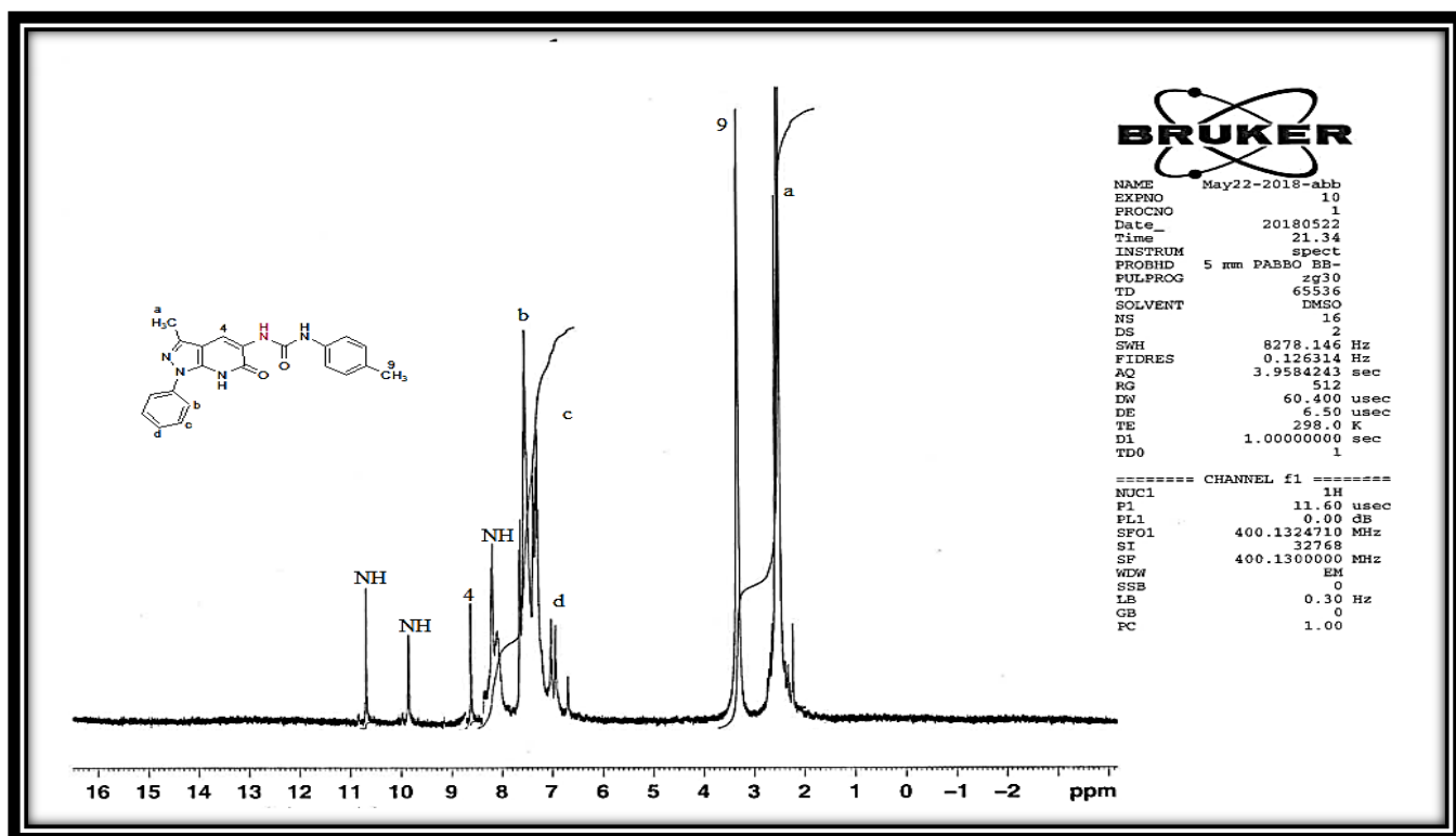
Figure 63. 1 H NMR spectrum of compound 20
