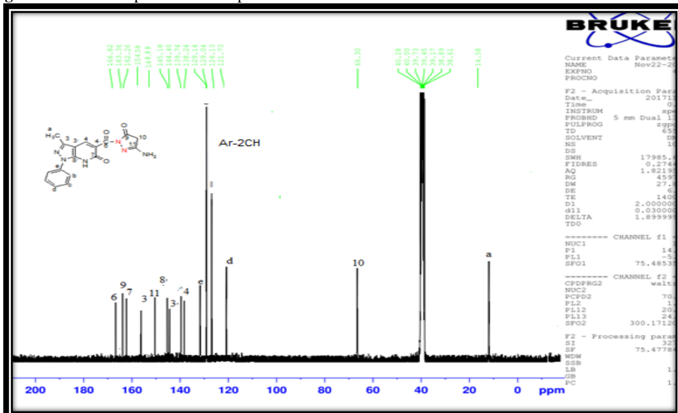
Figure 58. ^{13}\text{C} NMR spectrum of compound 16
