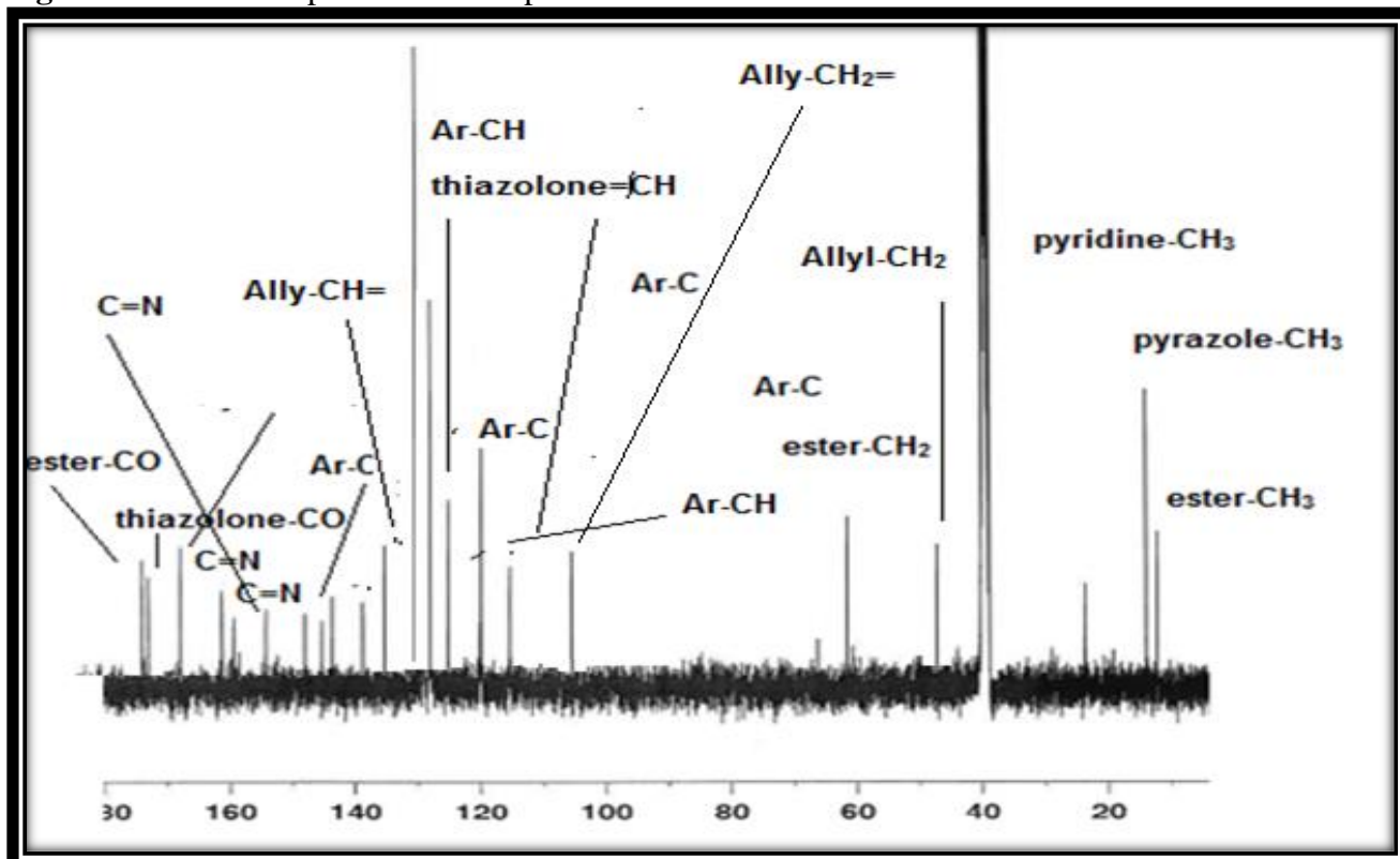
Figure 56. ^{13}\text{C} NMR spectrum of compound 14b
