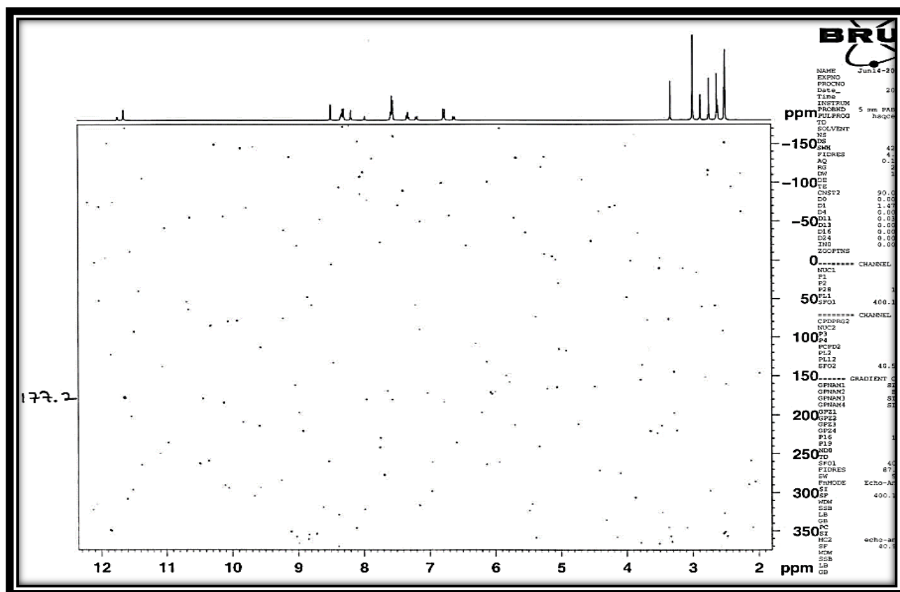
Figure 25. ^1\text{H} - ^{15}\text{N} HSQC spectrum of compound 8b
