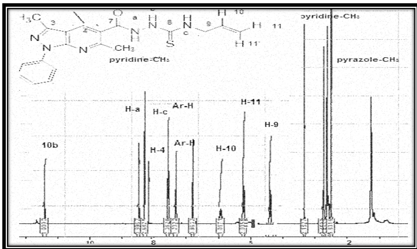
Figure 9. ^1\text{H} NMR of compound 6b
