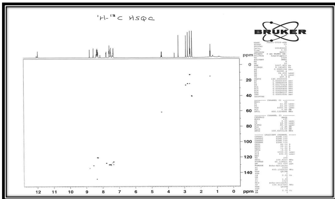
Figure 15. ^1\text{H} - ^{13}\text{C} HSQC spectrum of compound 8a
