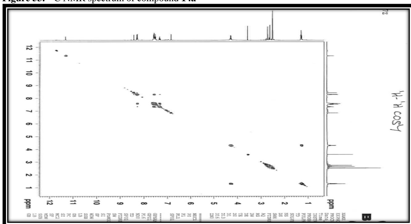
Figure 54. COSY ^1\text{H} - ^1\text{H} NMR spectrum of compound 14a
