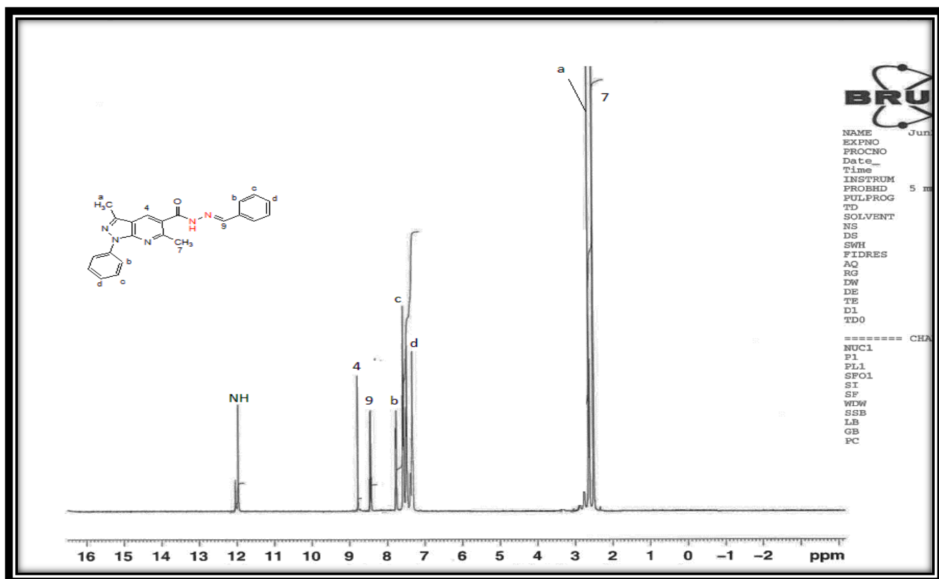
Figure 11. ^1\text{H} NMR spectrum of compound 8a
