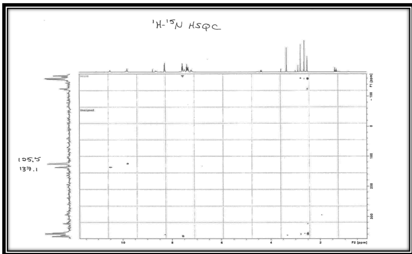
Figure 7. ^1\text{H} - ^{15}\text{N} HSQC spectrum of compound 6a
