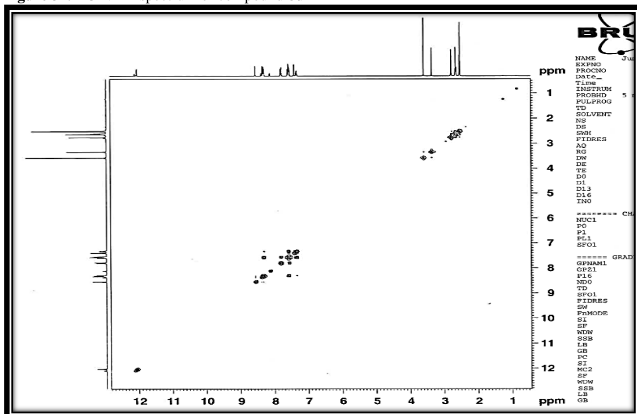
Figure 32. ^1\text{H} - ^1\text{H} COSY spectrum of compound 8d
