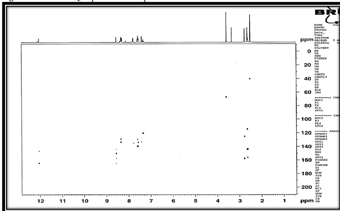
Figure 34. ^1\text{H} - ^{13}\text{C} HMBC spectrum of compound 8d
