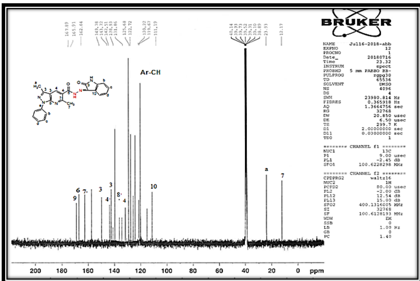
Figure 45. ^{13}\text{C} NMR spectrum of compound 8f
