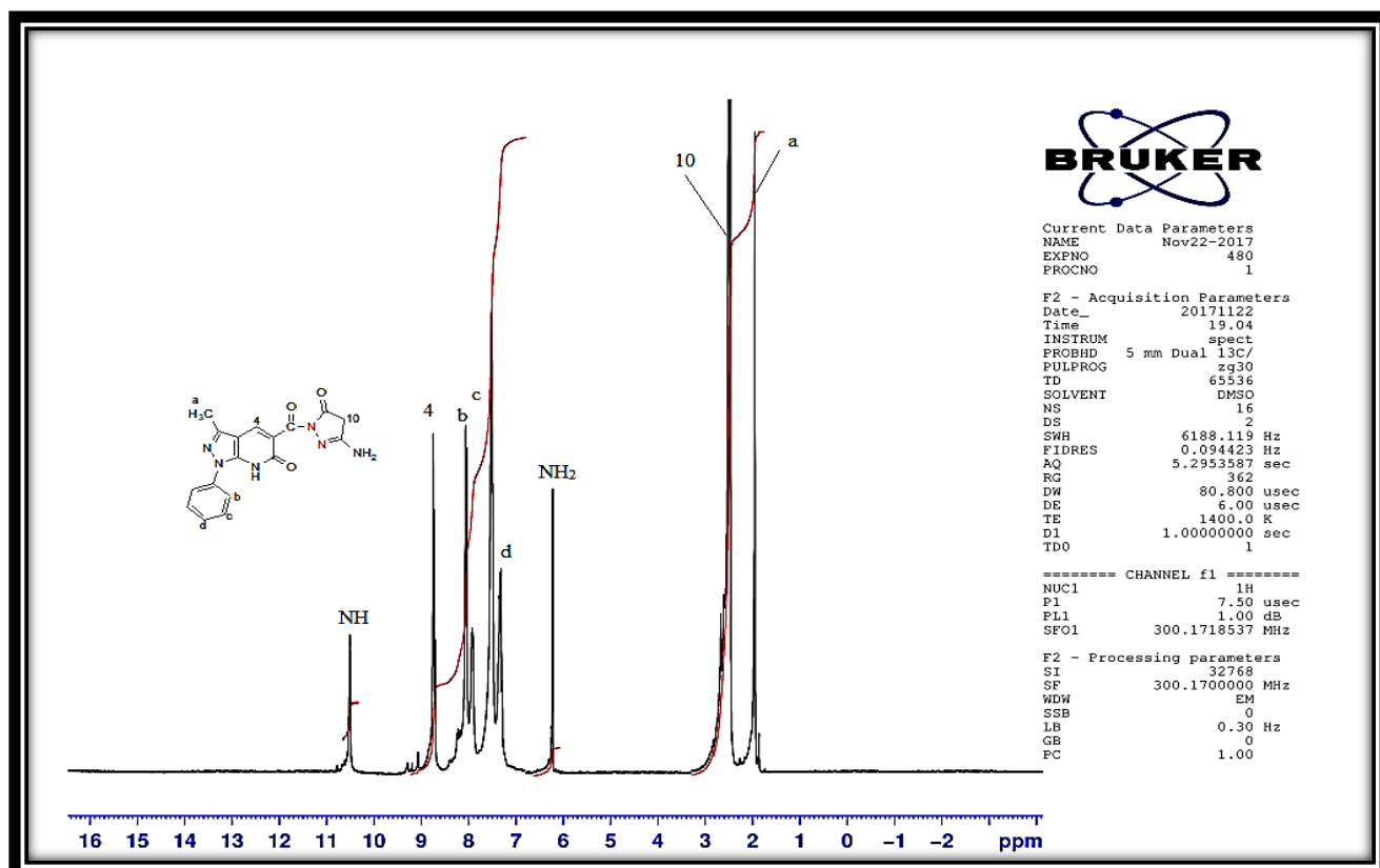
Figure 57. ^1\text{H} NMR spectrum of compound 16
