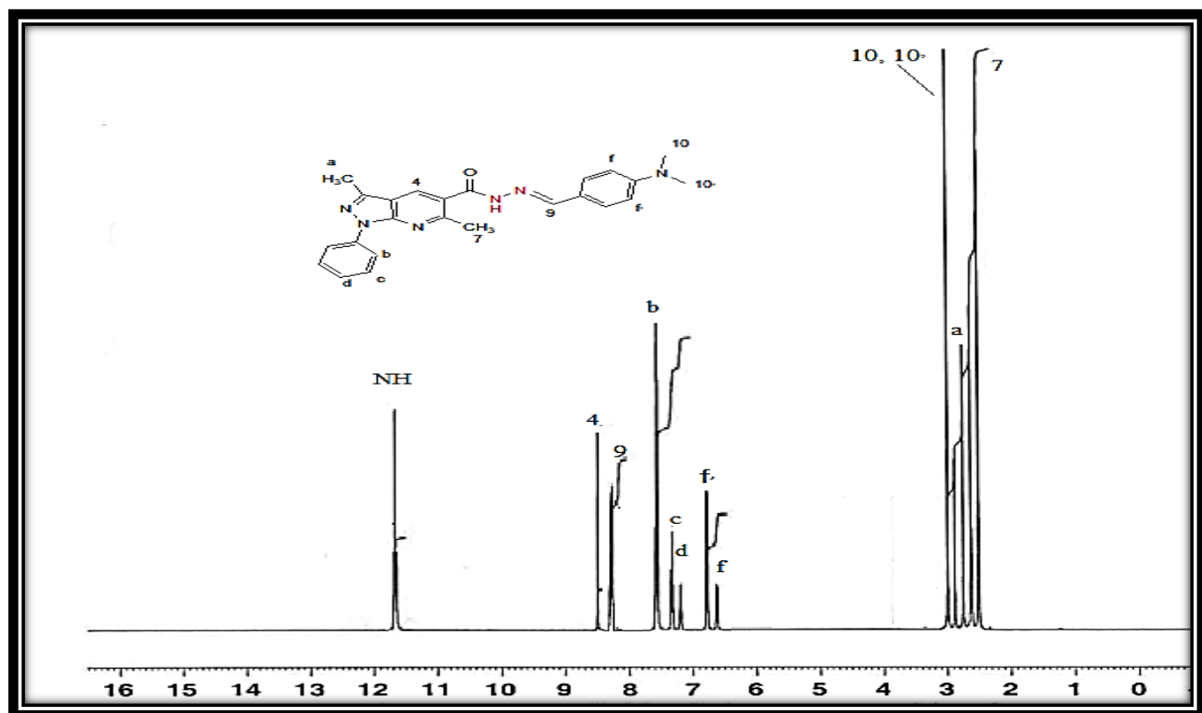
Figure 19. ^1\text{H} NMR spectrum of compound 8b
