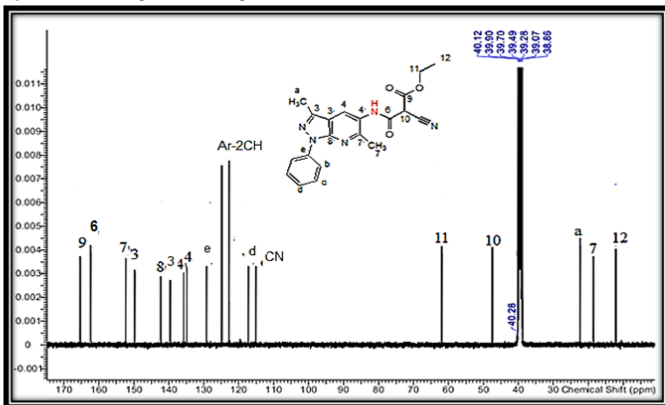
Figure 48. ^{13}\text{C} NMR spectrum of compound 11
