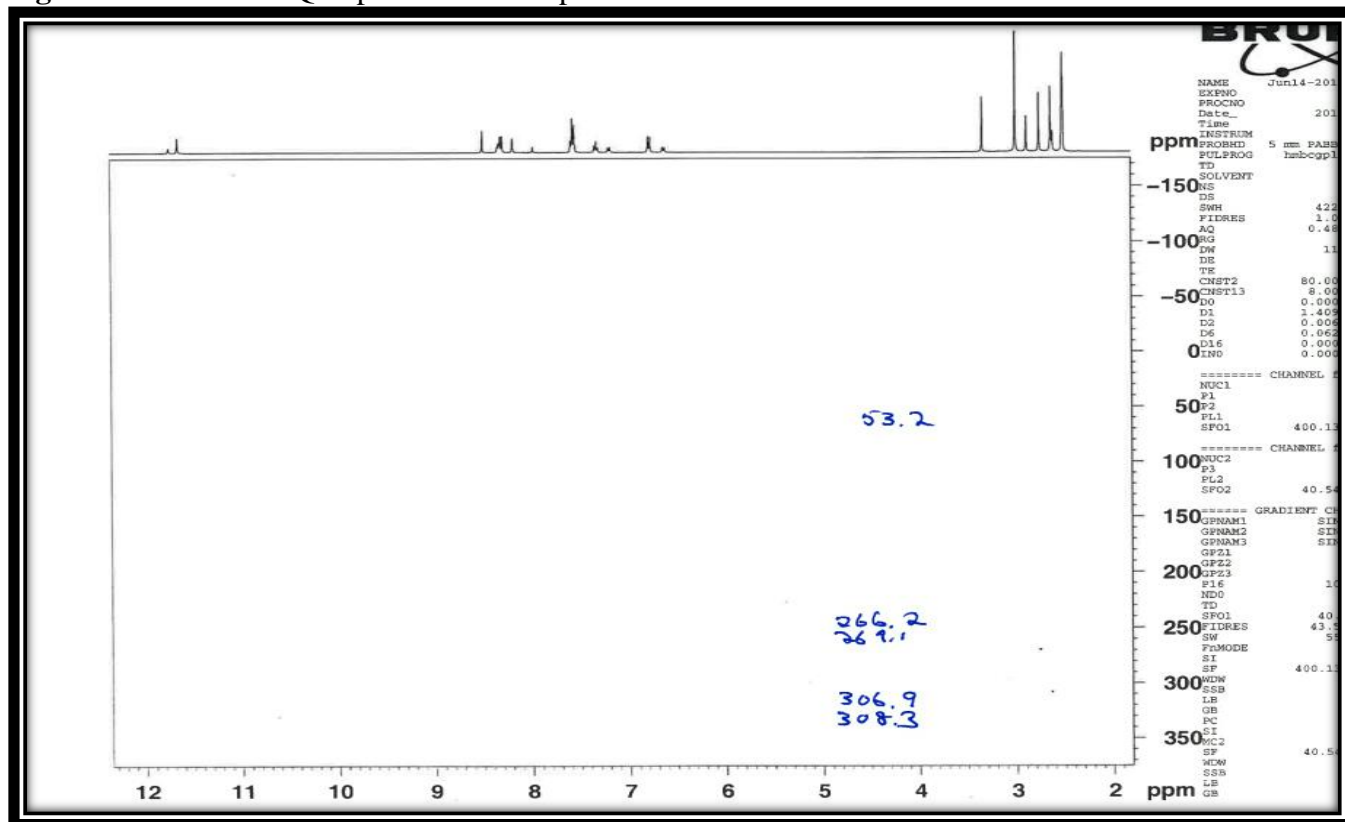
Figure 26. ^1\text{H} - ^{15}\text{N} HMBC spectrum of compound 8b
