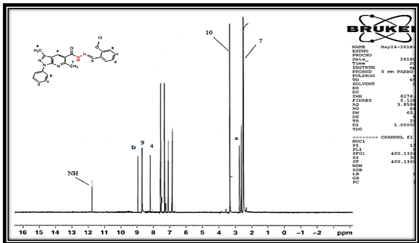
Figure 27. 1 H NMR spectrum of compound 8c
