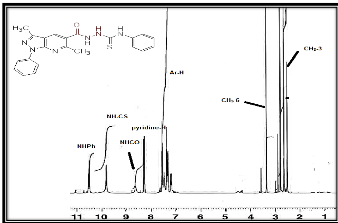
Figure 1. 1 H NMR spectrum of compound 6a
