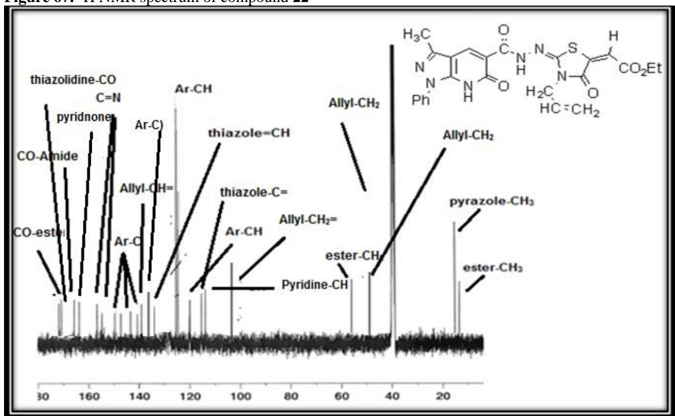
Figure 68. ^{13}\text{C} NMR spectrum of compound 22
