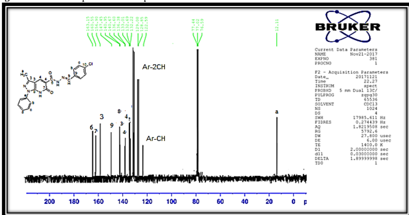
Figure 62. ^{13}\text{C} NMR spectrum of compound 18
