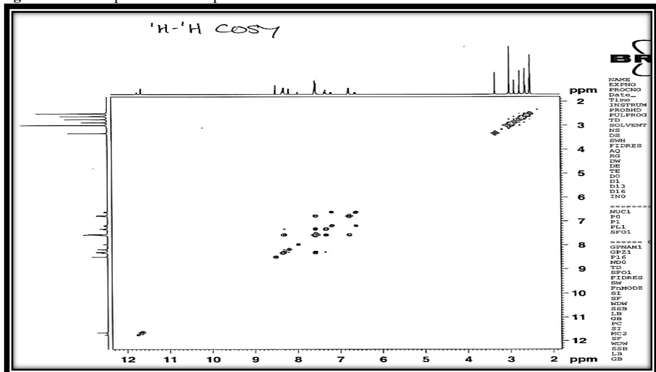
Figure 22. 1 H- 1 H COSY spectrum of compound 8b
