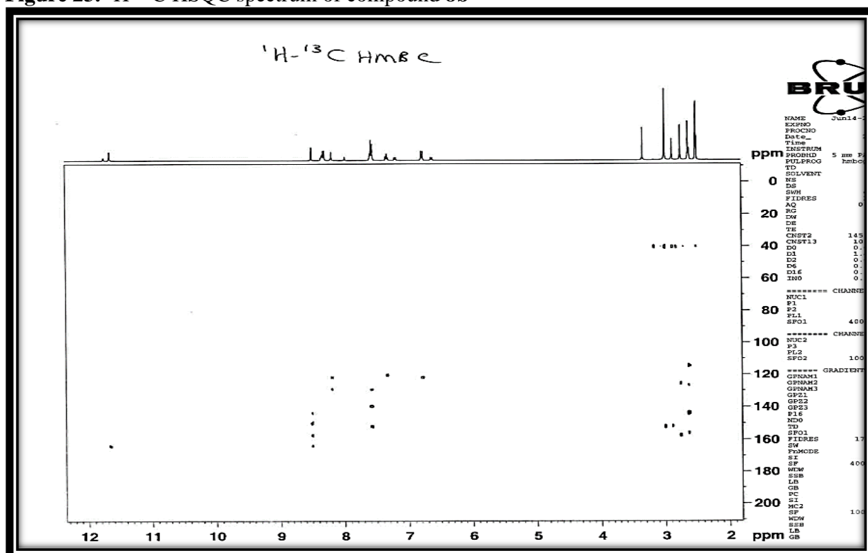
Figure 24. ^1\text{H} - ^{13}\text{C} HMBC spectrum of compound 8b
