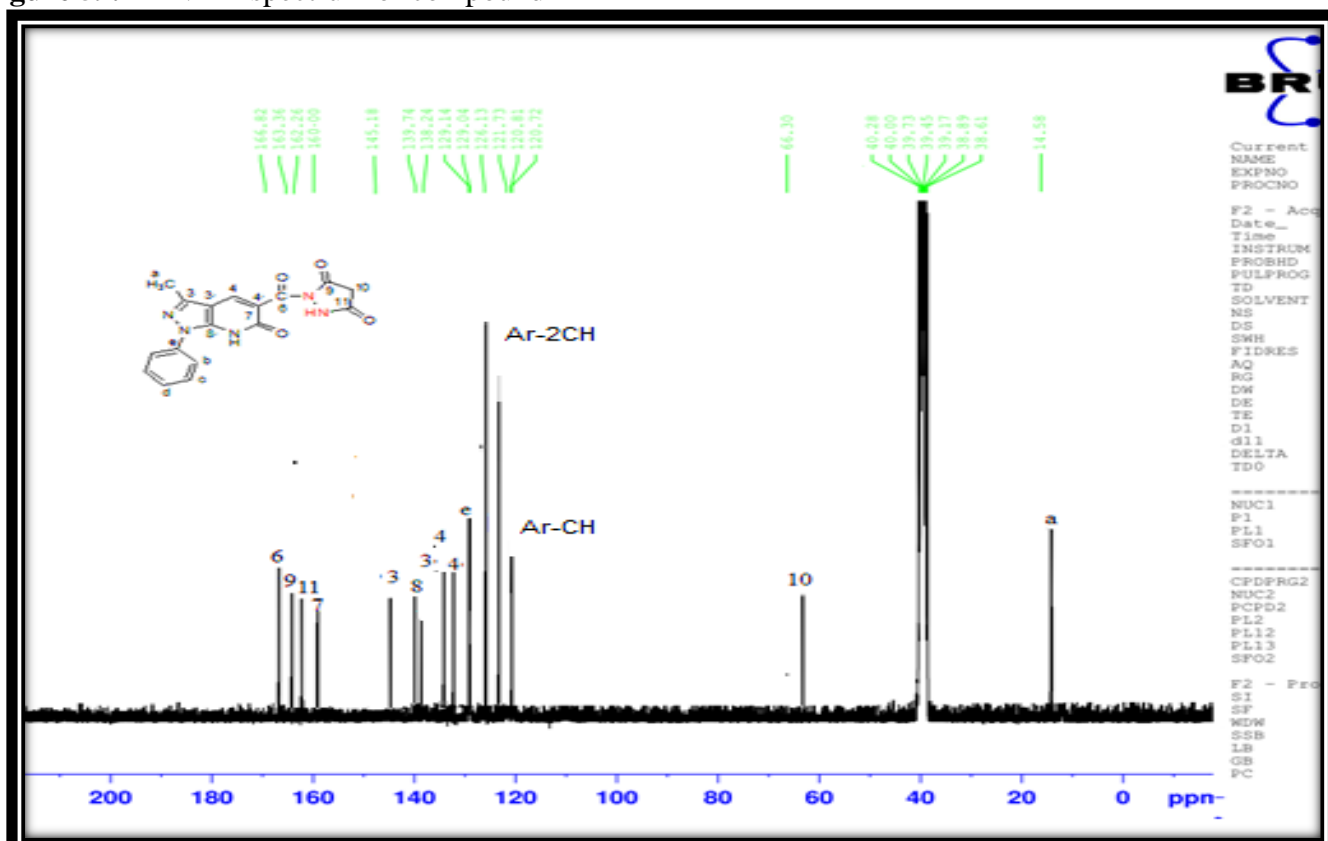
Figure 60. ^{13}\text{C} NMR spectrum of compound 17
