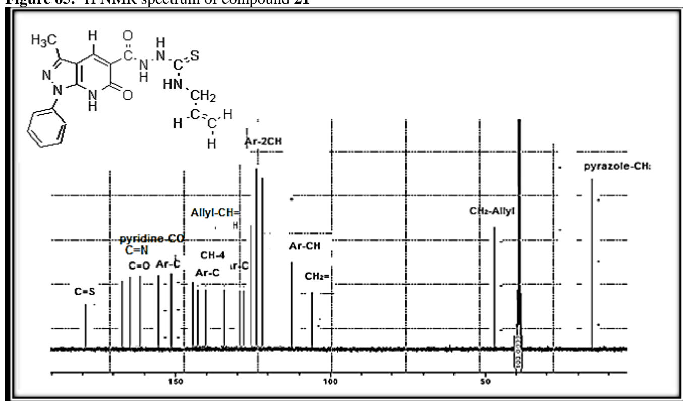
Figure 66. ^{13}\text{C} NMR spectrum of compound 21
