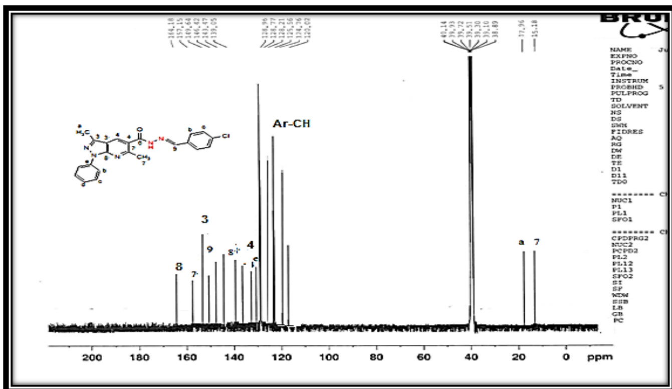
Figure 31. ^{13}\text{C} NMR spectrum of compound 8d
