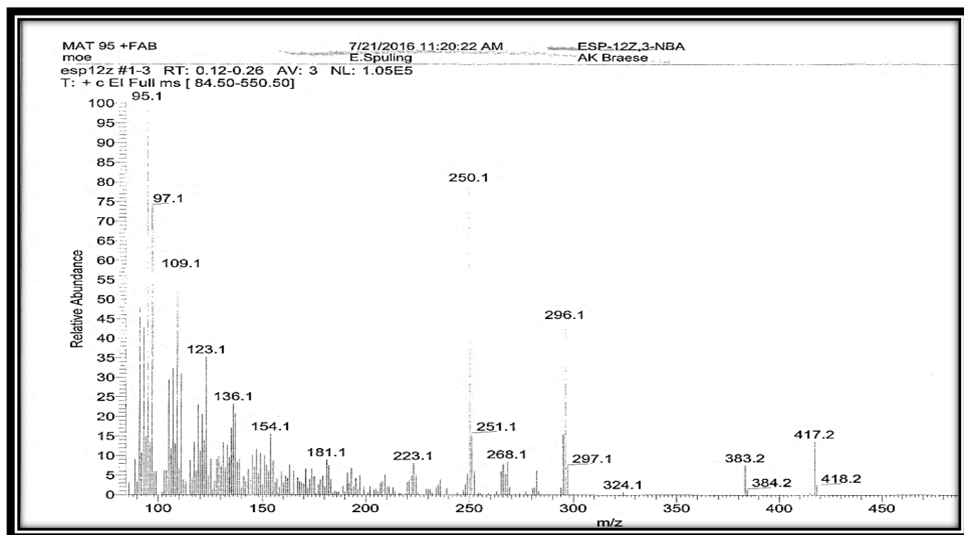
Figure 3. Mass spectrum of compound 6a
