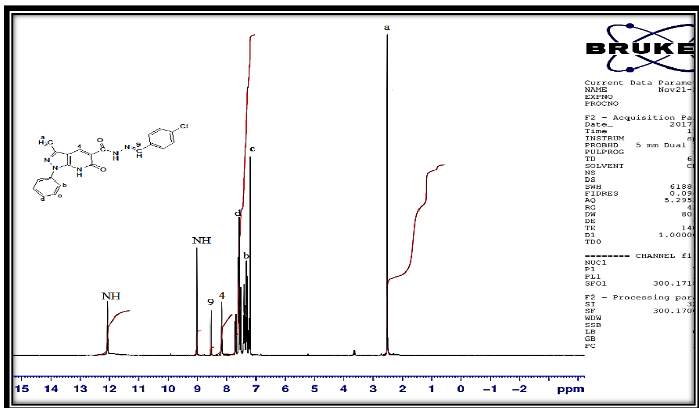
Figure 61. ^1\text{H} NMR spectrum of compound 18
