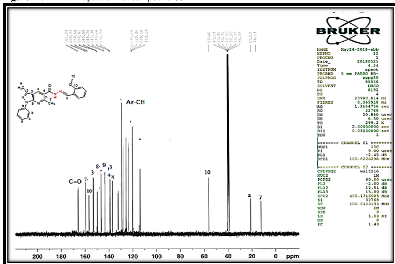
Figure 28. 13 C NMR spectrum of compound 8c
