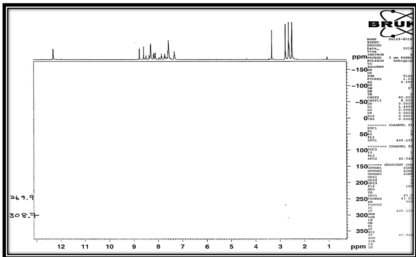
Figure 43. ^1\text{H} - ^{15}\text{N} HMBC spectrum of compound 8e
