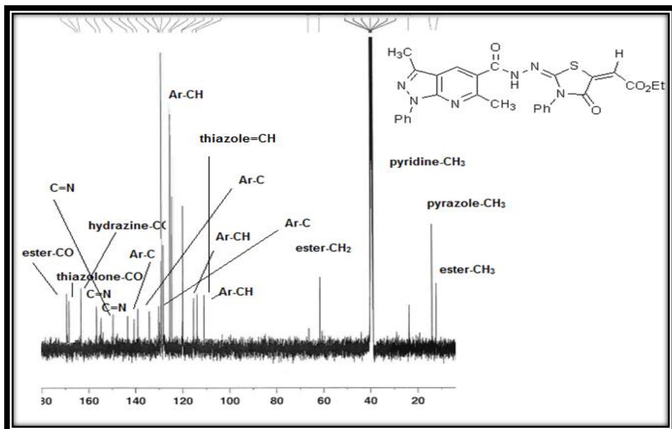
Figure 53. ^{13}\text{C} NMR spectrum of compound 14a
