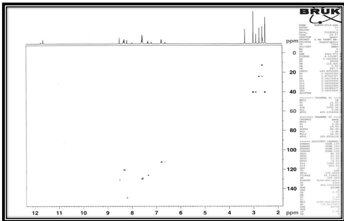
Figure 23. ^1\text{H} - ^{13}\text{C} HSQC spectrum of compound 8b
