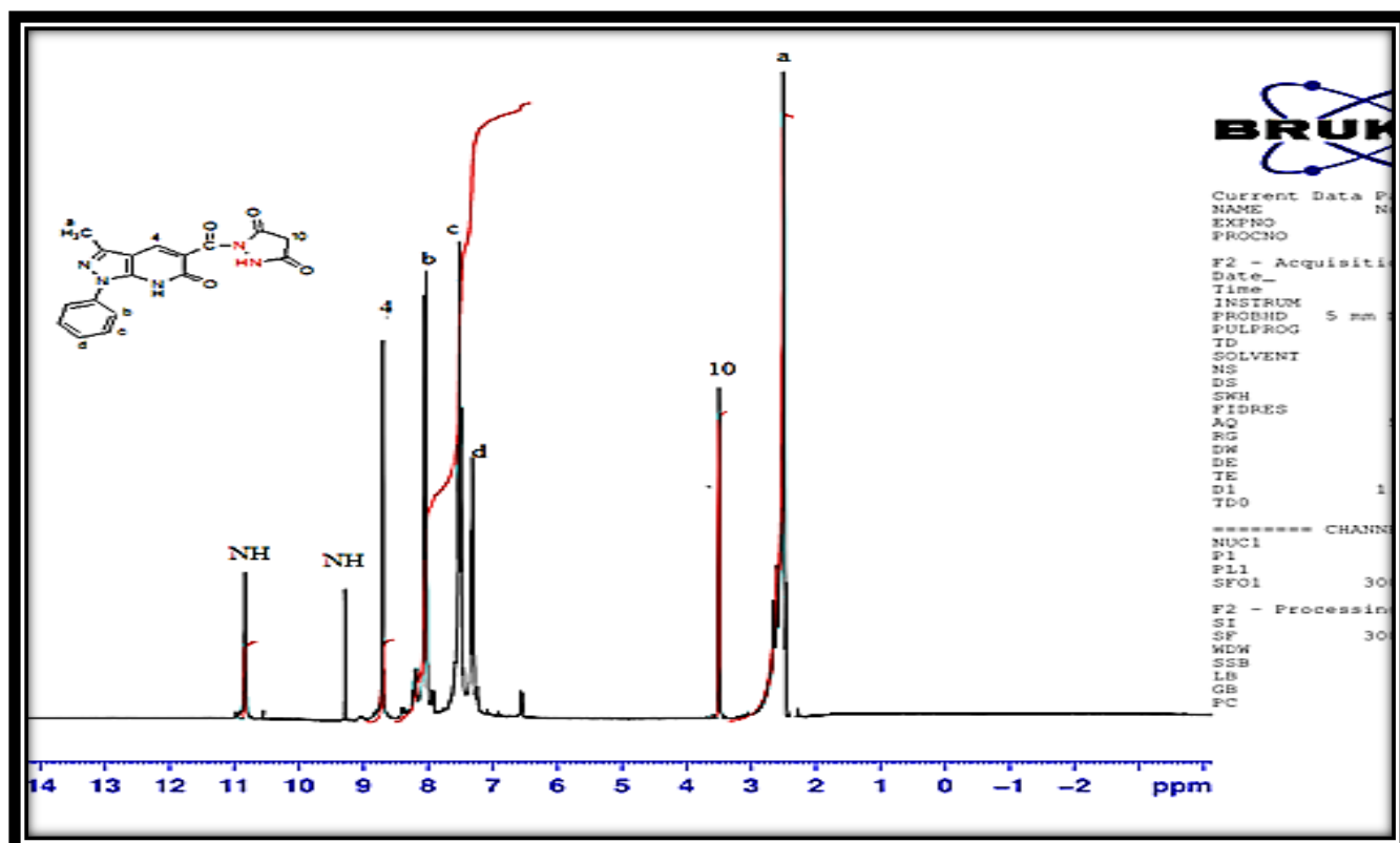
Figure 59. ^1\text{H} NMR spectrum of compound 17
