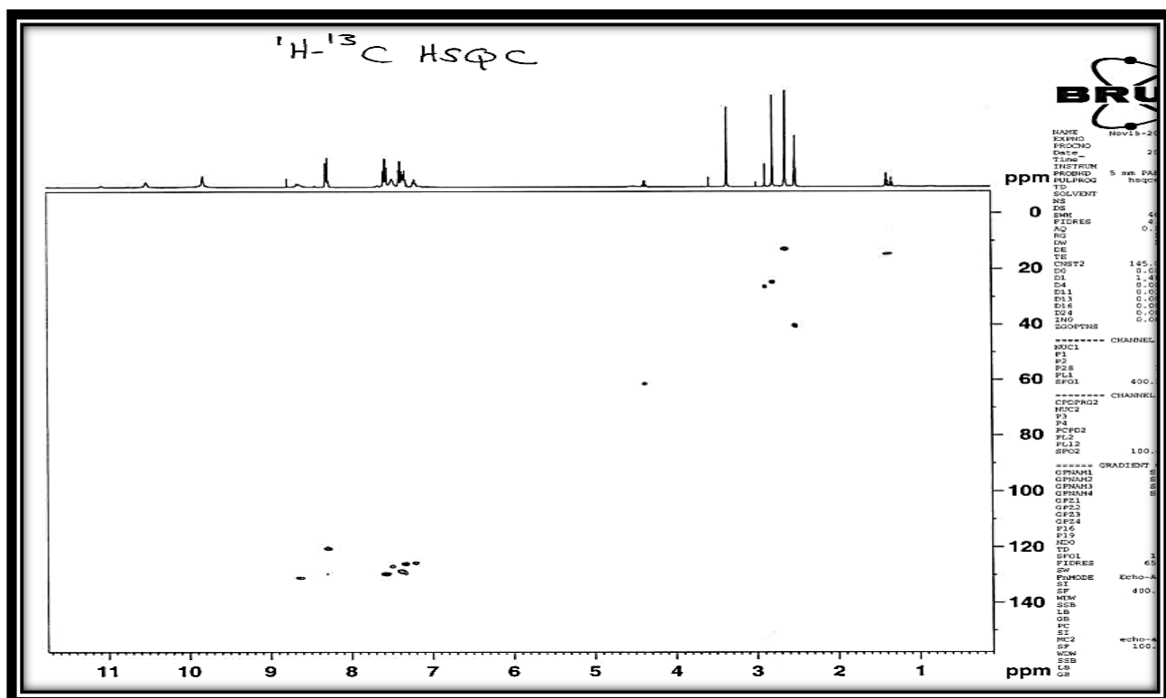
Figure 5. ^1\text{H} - ^{13}\text{C} HSQC spectrum of compound 6a
