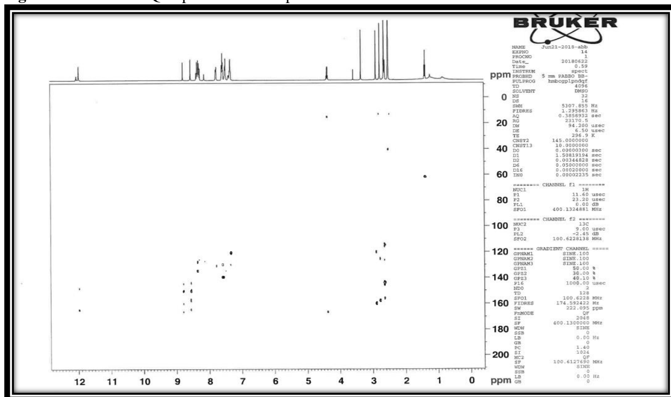
Figure 16. ^1\text{H} - ^{13}\text{C} HMBC spectrum of compound 8a
