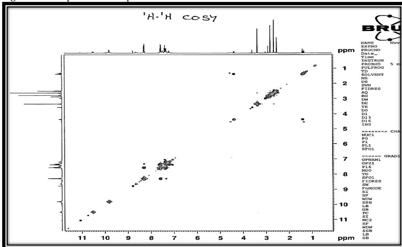
Figure 4. ^1\text{H} - ^1\text{H} COSY spectrum of compound 6a
