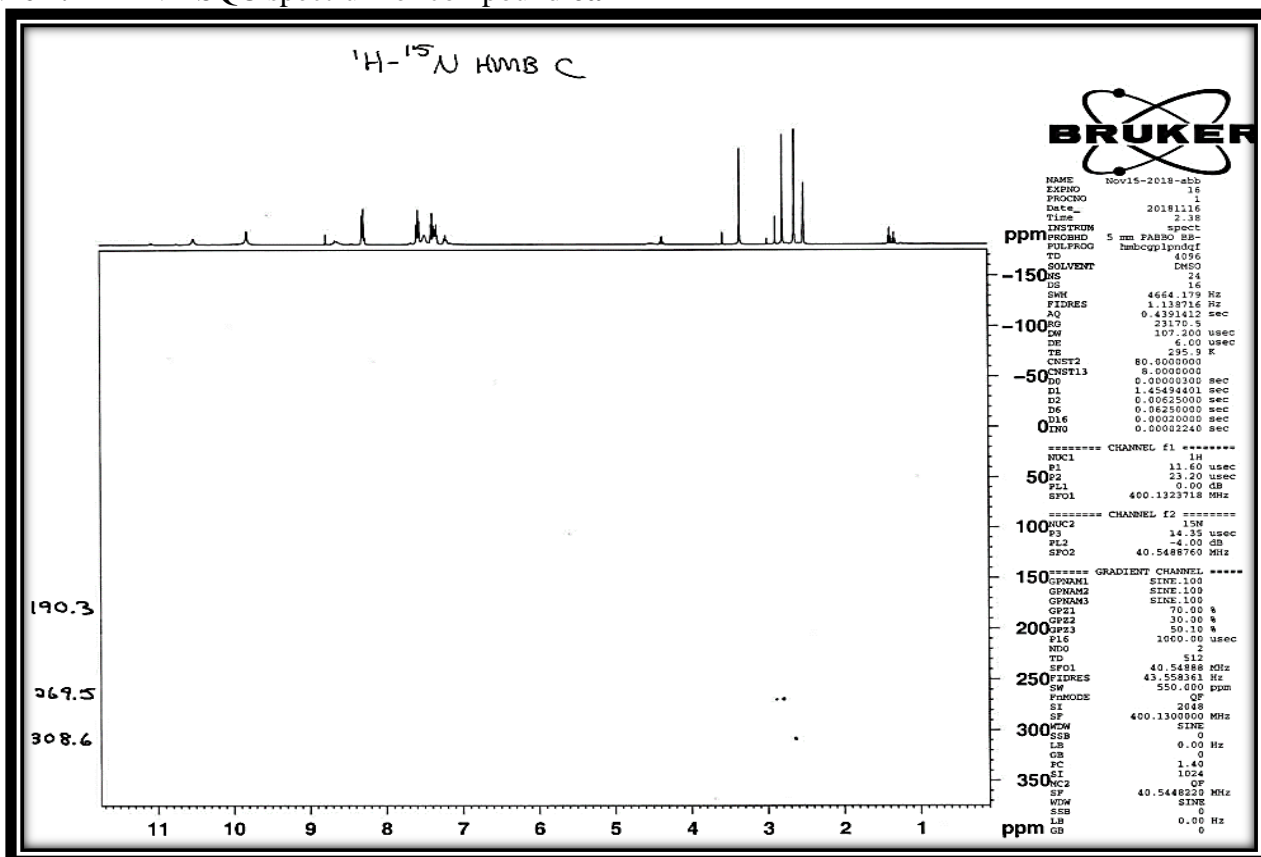
Figure 8. ^1\text{H} - ^{15}\text{N} HMB C spectrum of compound 6a
