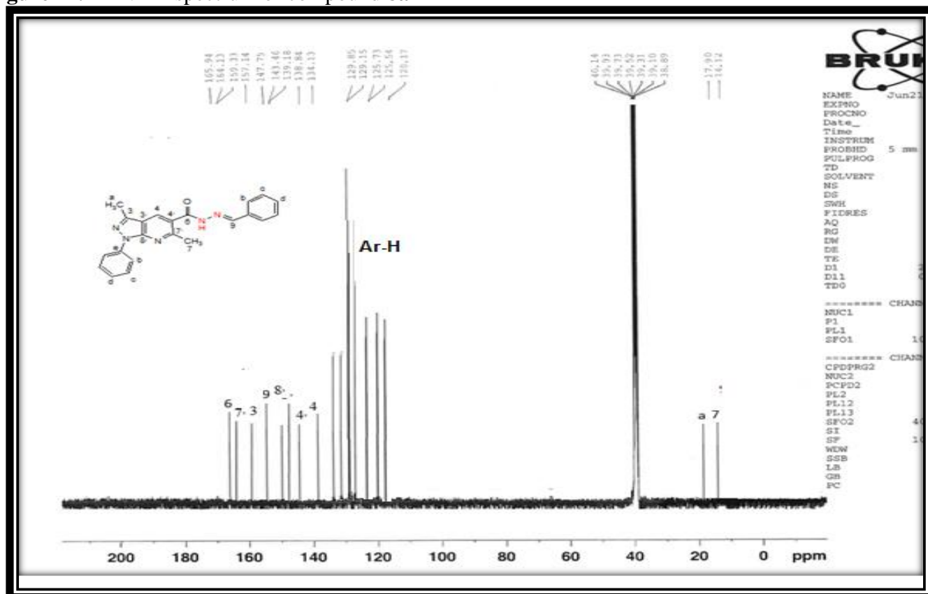
Figure 12. ^{13}\text{C} NMR spectrum of compound 8a
