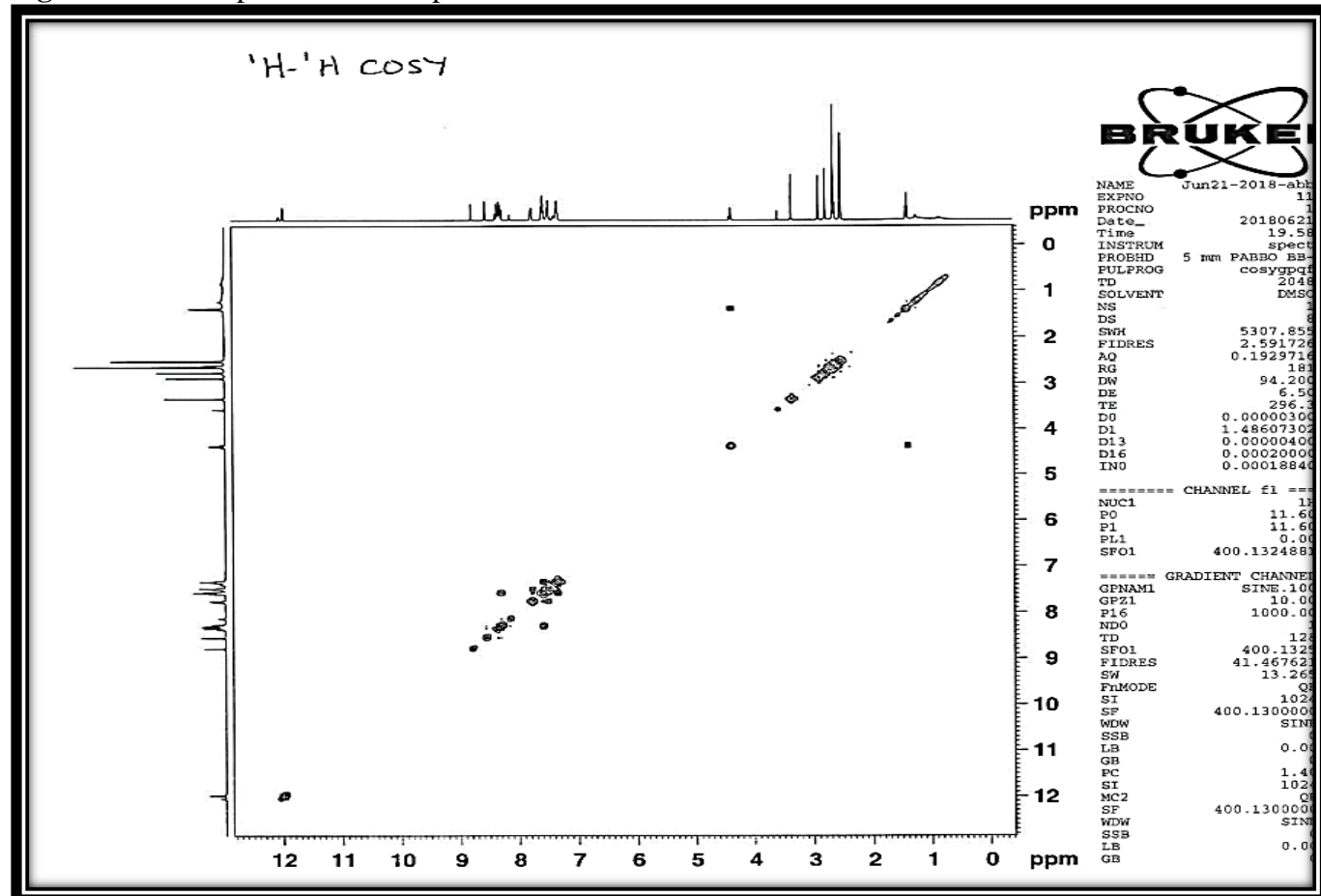
Figure 14. 1 H- 1 H COSY spectrum of compound 8a
