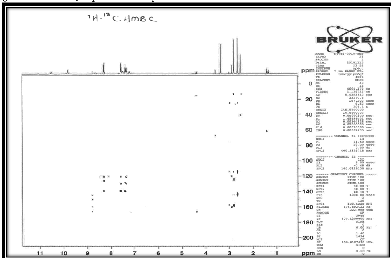
Figure 6. ^1\text{H} - ^{13}\text{C} HMBC spectrum of compound 6a
