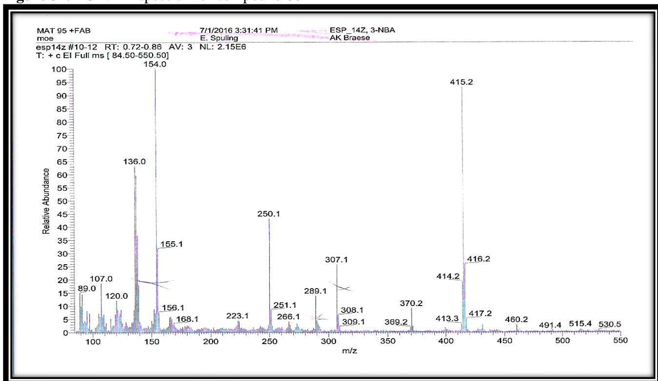
Figure 38. Mass spectrum of compound 8e
