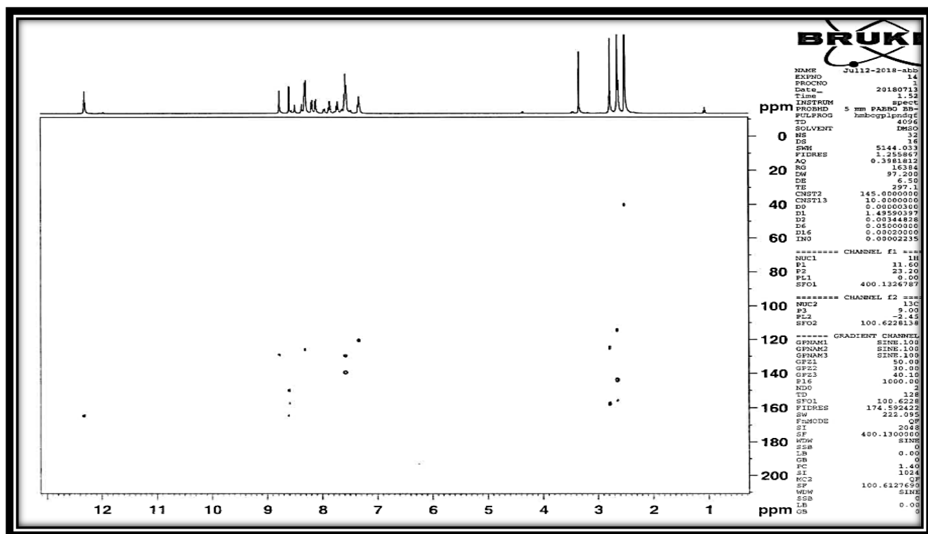
Figure 41. ^1\text{H} - ^{13}\text{C} HMBC spectrum of compound 8e
