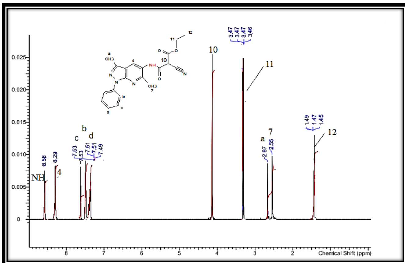
Figure 47. ^1\text{H} NMR spectrum of compound 11
