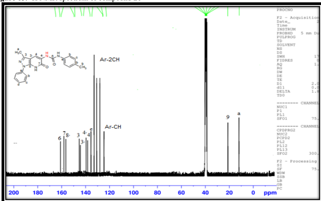
Figure 64. 13 C NMR spectrum of compound 20
