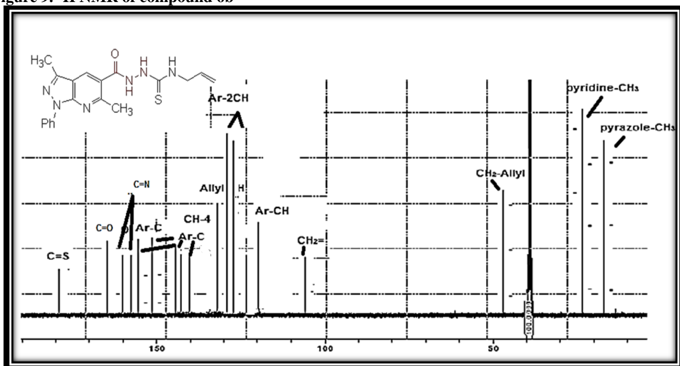
Figure 10. ^{13}\text{C} NMR of compound 6b
