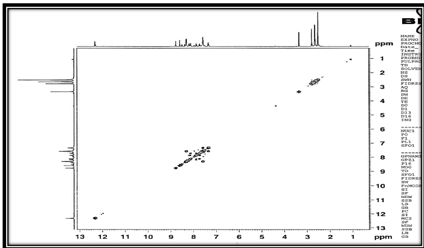
Figure 39. ^1\text{H} - ^1\text{H} COSY spectrum of compound 8e
