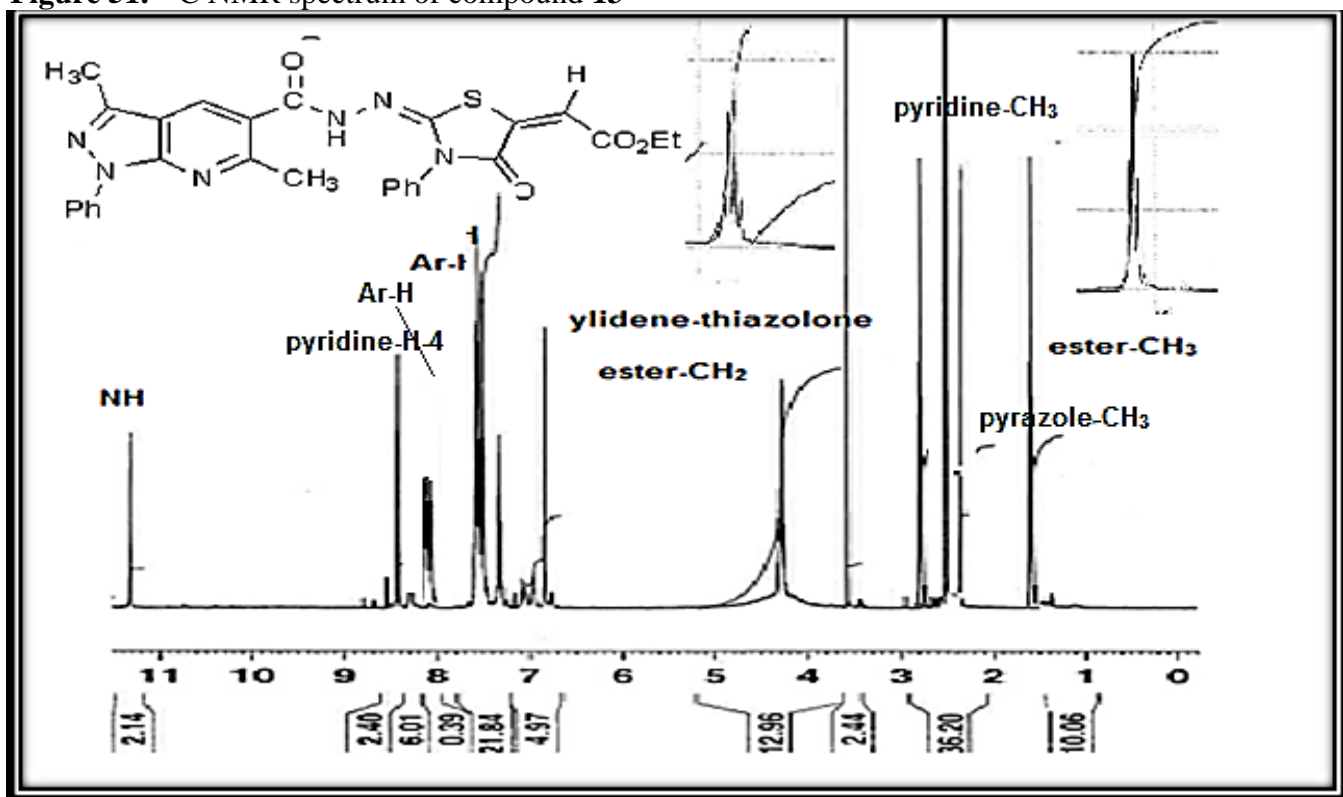
Figure 52. 1 H NMR spectrum of compound 14a
