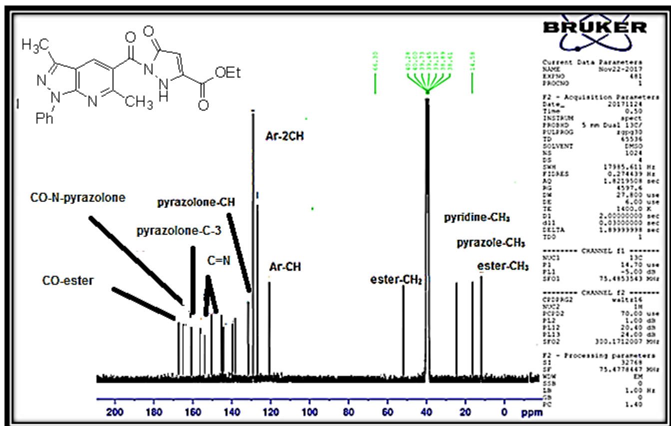
Figure 51. 13 C NMR spectrum of compound 13
