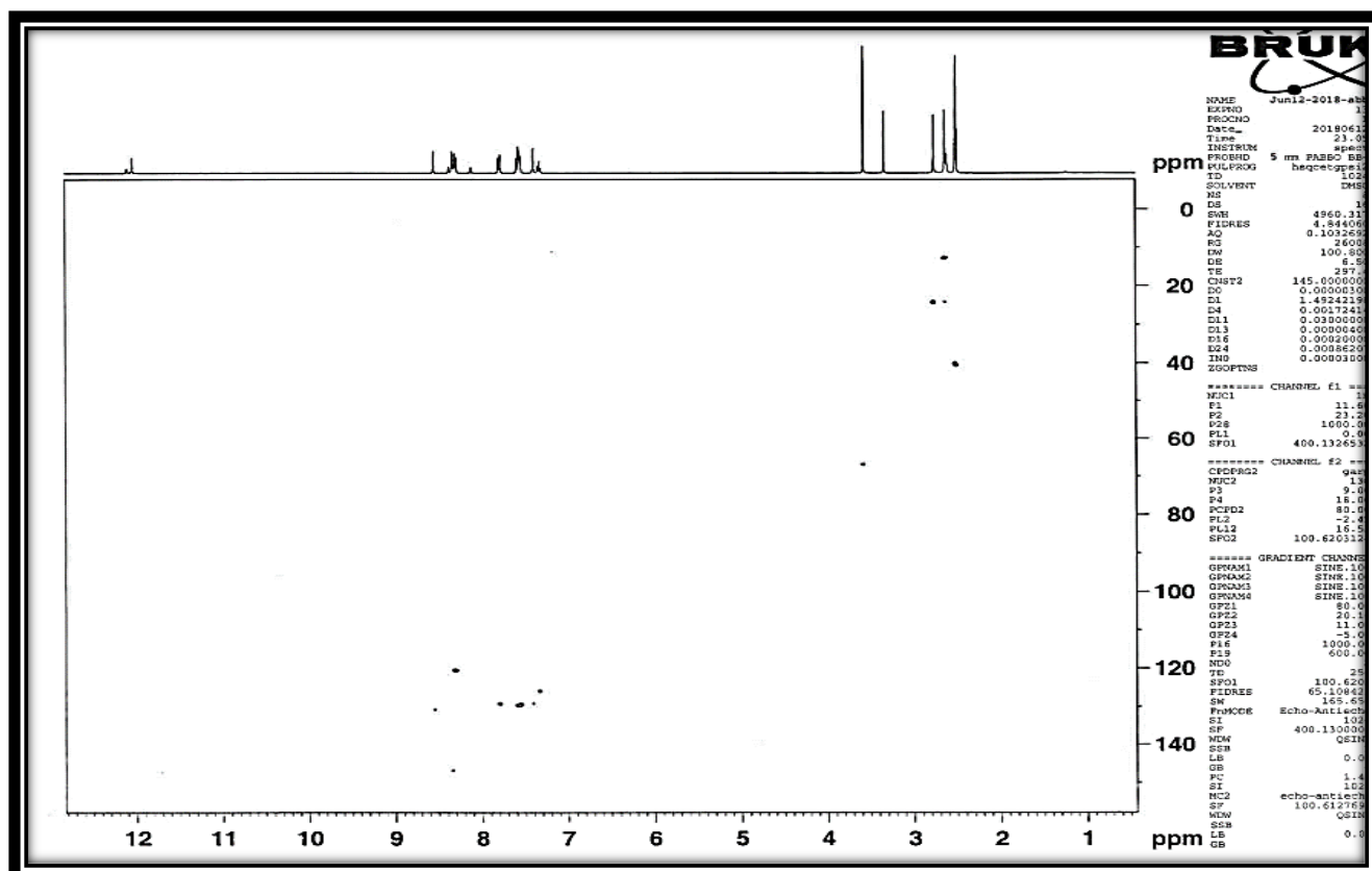
Figure 33. ^1\text{H} - ^{13}\text{C} HSQC spectrum of compound 8d
