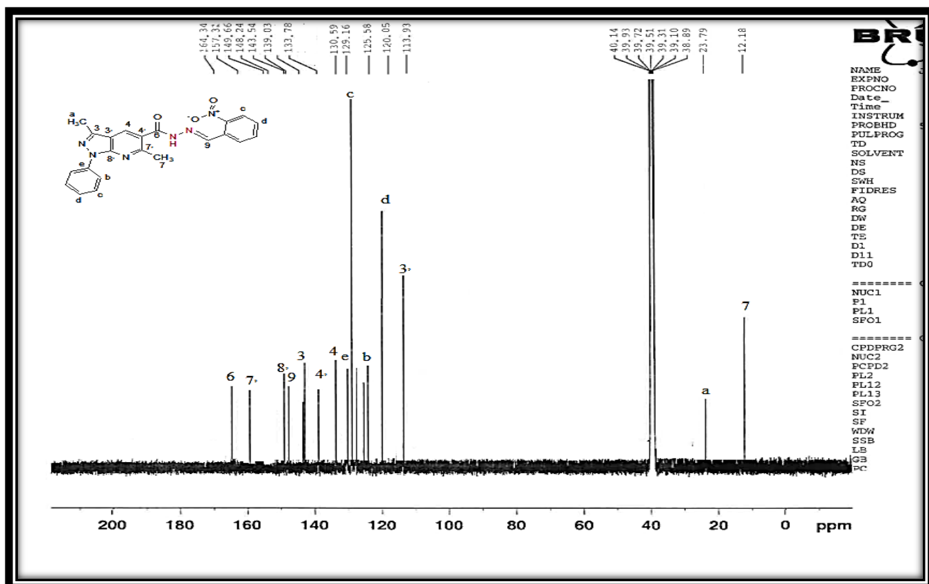
Figure 37. ^{13}\text{C} NMR spectrum of compound 8e
