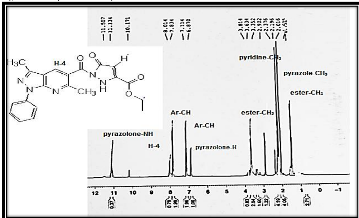
Figure 50. 1 H NMR spectrum of compound 13
