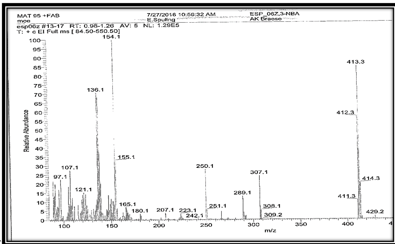
Figure 21. Mass spectrum of compound 8b
