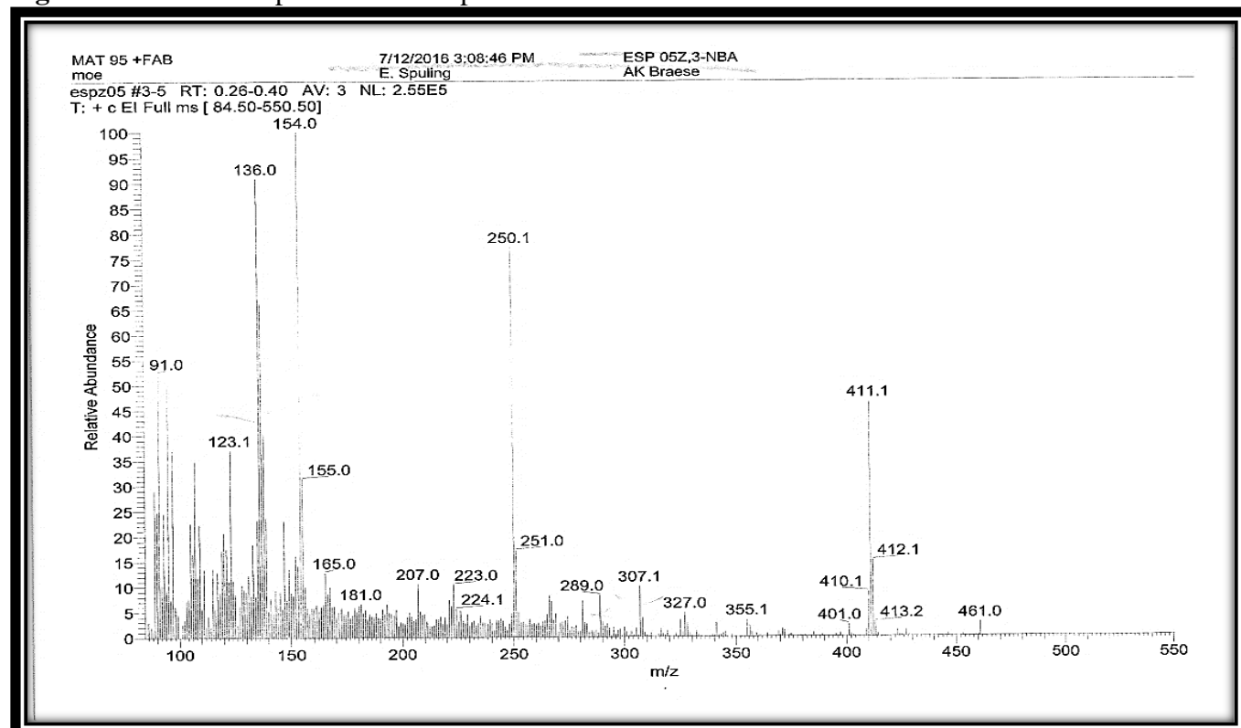
Figure 46. Mass spectrum of compound 8f
