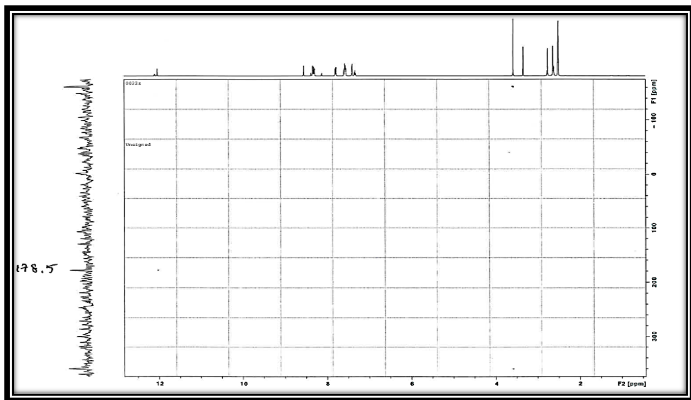
Figure 35. ^1\text{N} - ^{15}\text{N} HSQC spectrum of compound 8d
