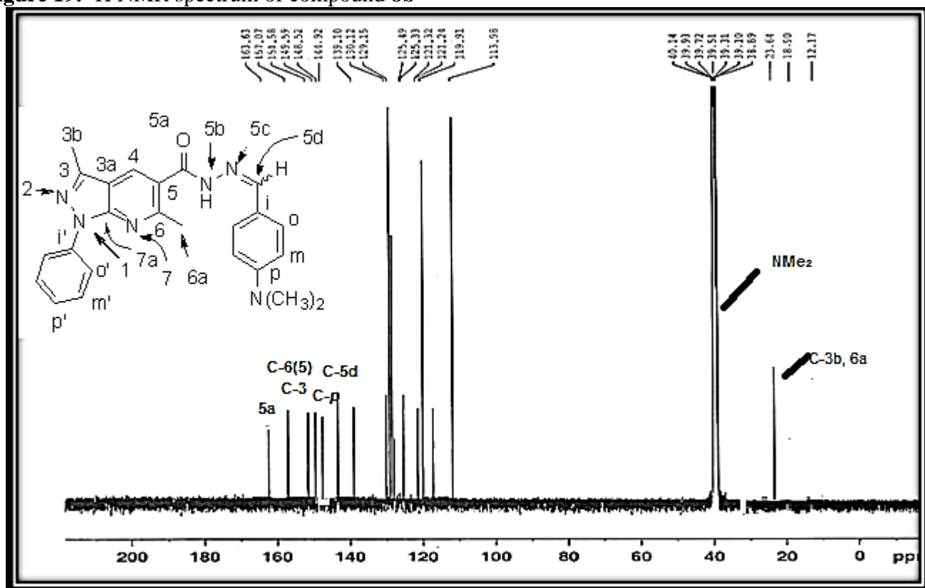
Figure 20. ^{13}\text{C} NMR spectrum of compound 8b
