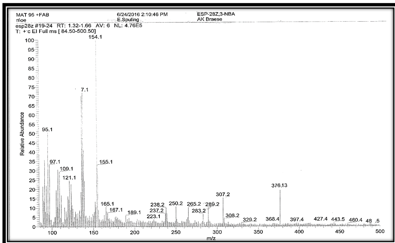
Figure 49. MS spectrum of compound 11
