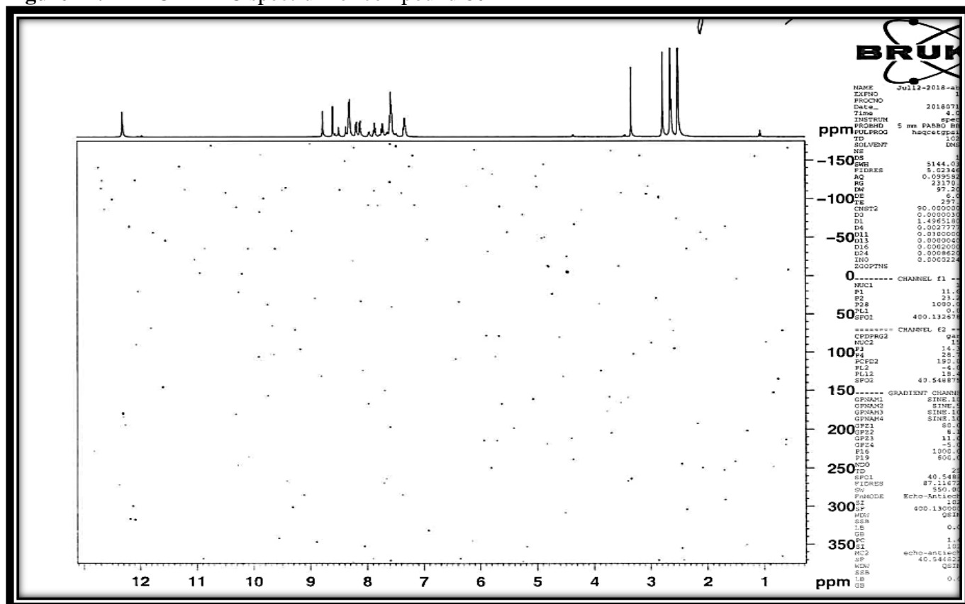
Figure 42. ^1\text{H} - ^{15}\text{N} HSQC spectrum of compound 8e
