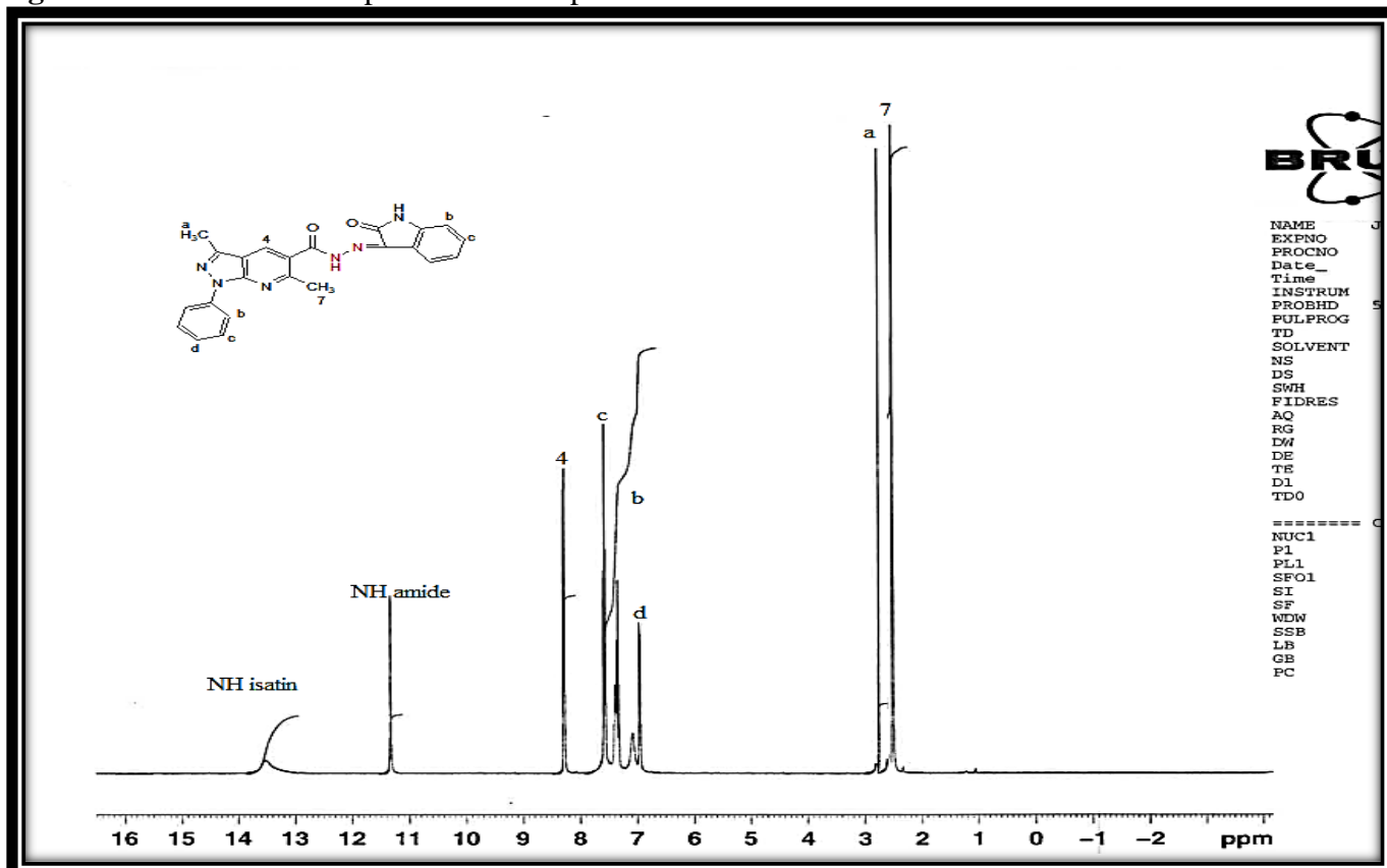
Figure 44. ^1\text{H} NMR spectrum of compound 8f
