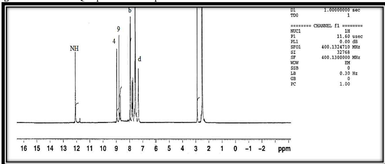
Figure 36. ^1\text{H} NMR spectrum of compound 8e
