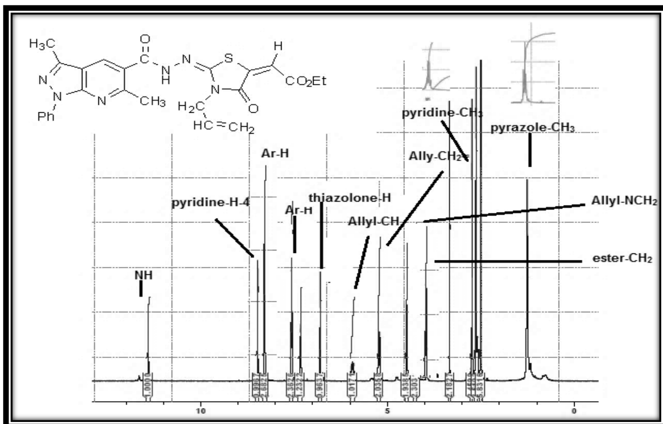
Figure 55. ^1\text{H} NMR spectrum of compound 14b
