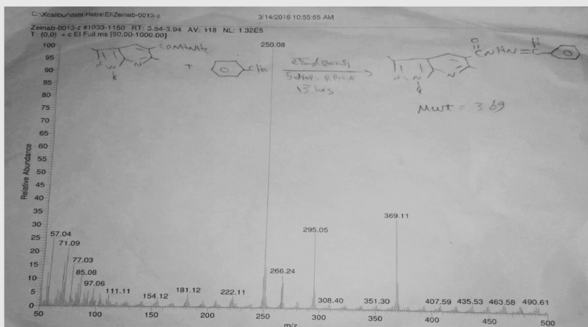
Figure 13. Mass spectrum of compound 8a
