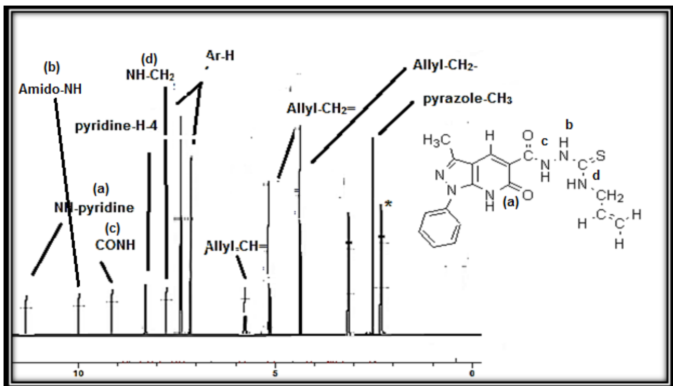
Figure 65. ^1\text{H} NMR spectrum of compound 21
