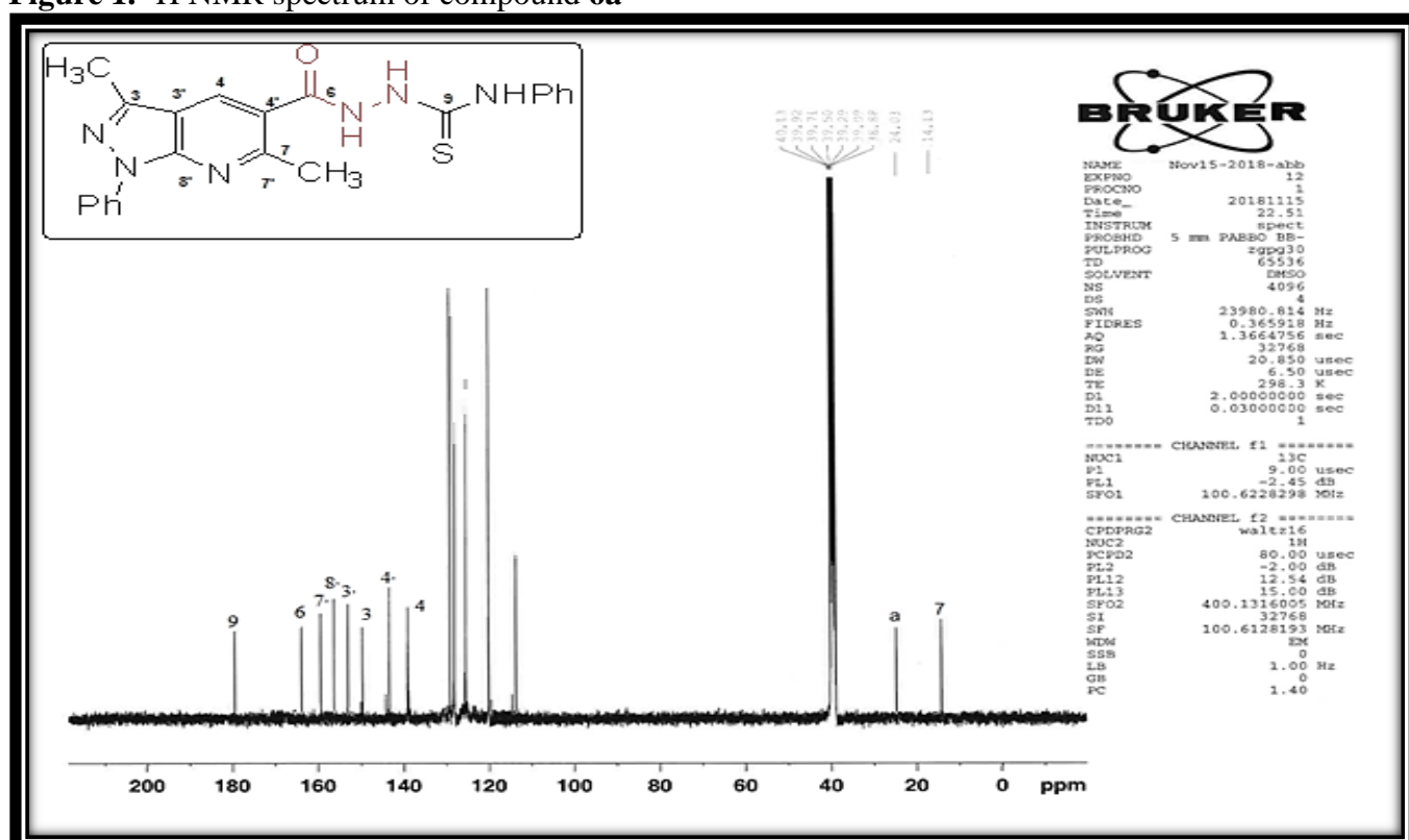
Figure 2. 13 C NMR spectrum of compound 6a
