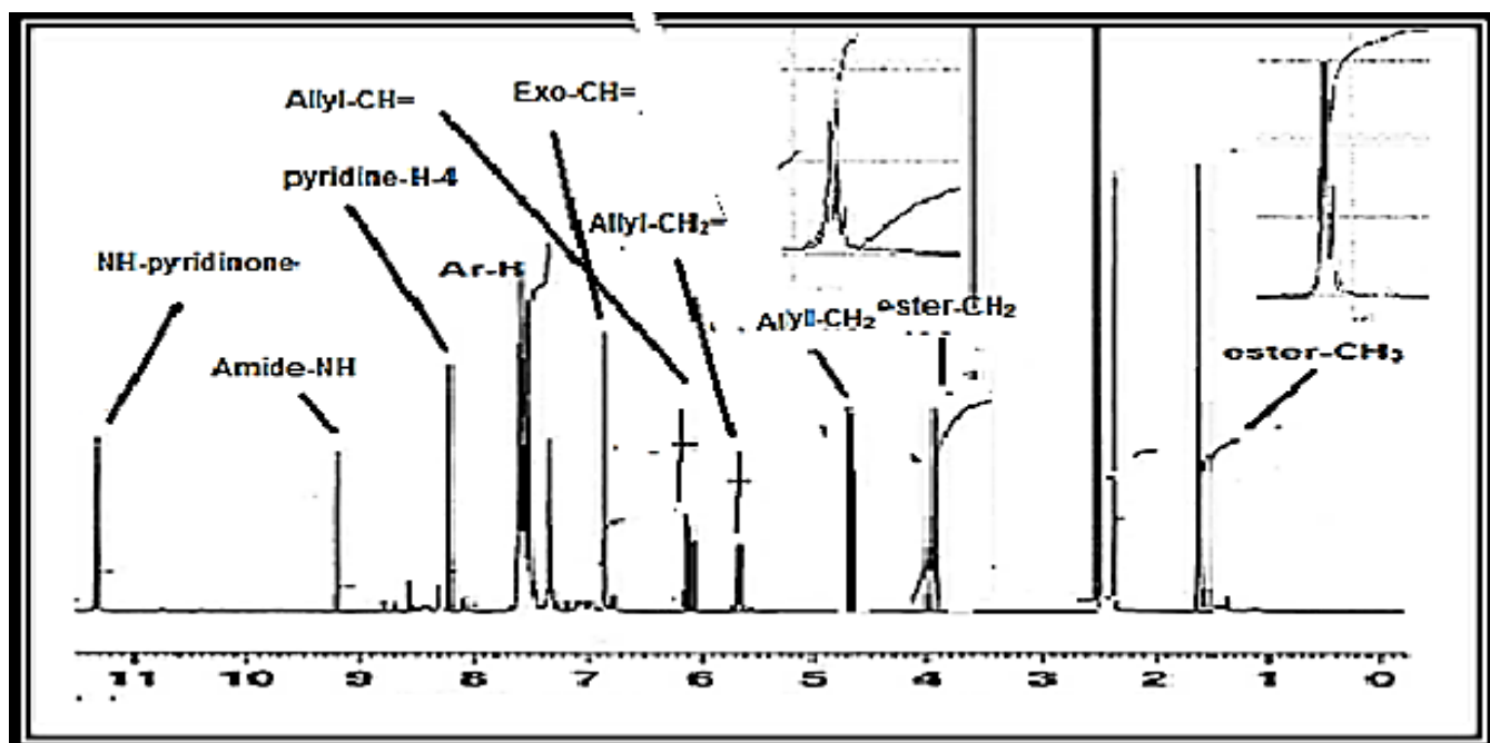
Figure 67. ^1\text{H} NMR spectrum of compound 22
