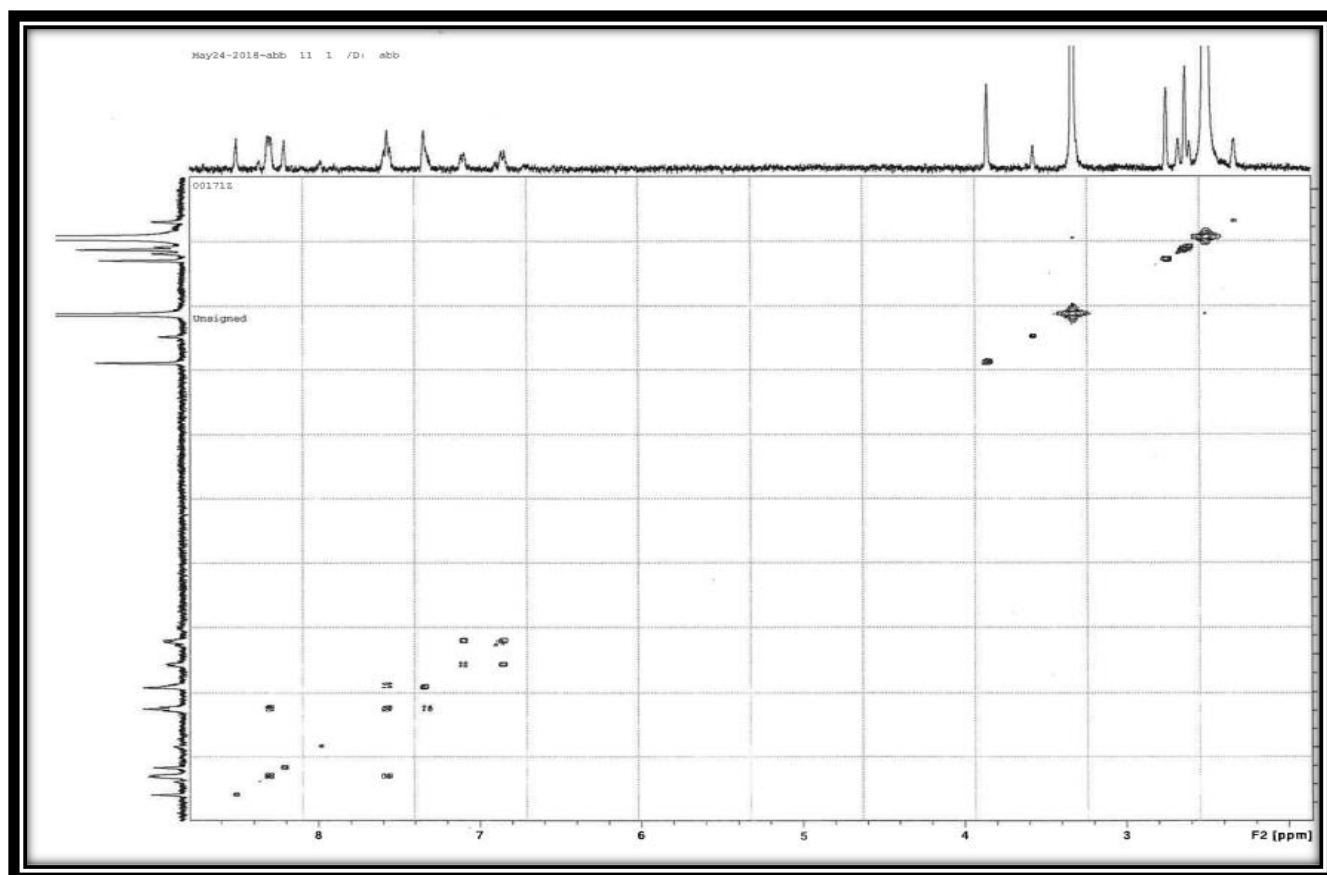
Figure 29. ^1\text{H} - ^1\text{H} COSY spectrum of compound 8c
