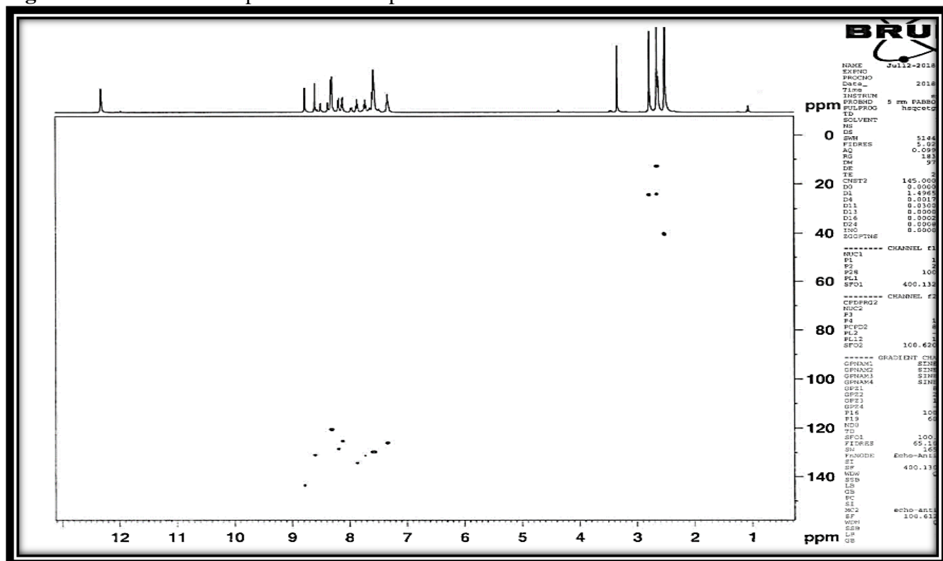
Figure 40. ^1\text{H} - ^{13}\text{C} HSQC spectrum of compound 8e
