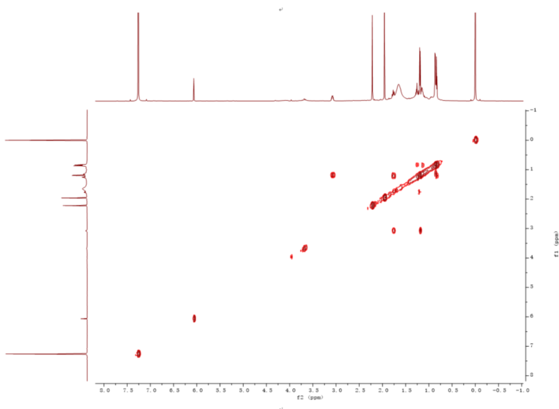
Figure S8. 1 H- 1 H COSY spectrum of compound 1 in CDCl 3 .
