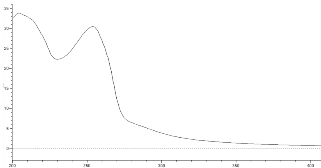
Figure S2. UV spectrum of 1
