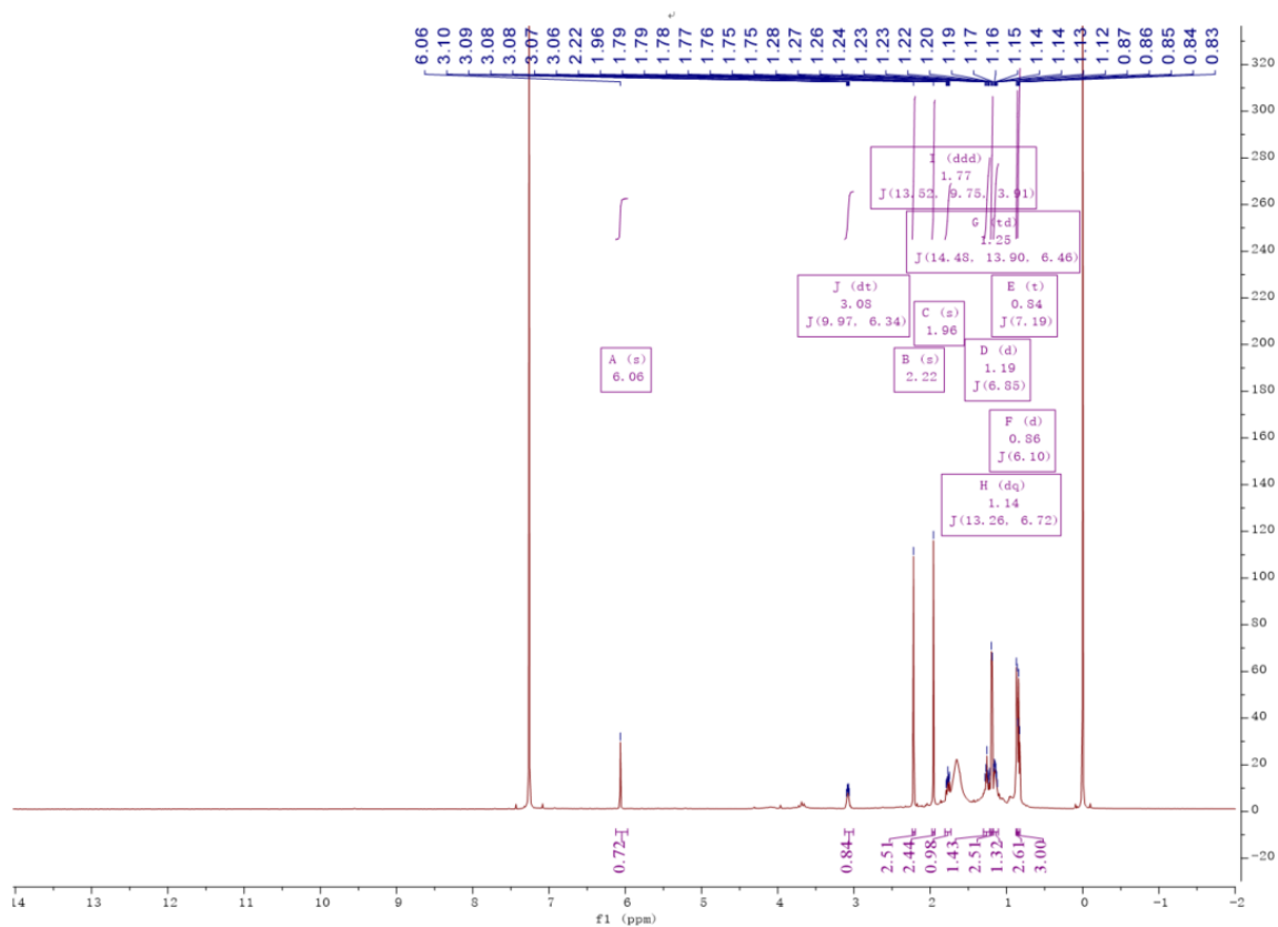
Figure S4. 1 H NMR spectrum of compound 1 in CDCl 3 .
