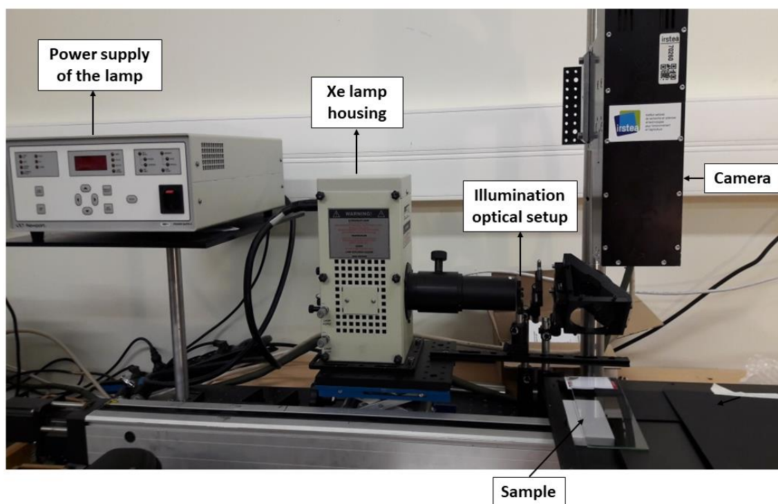
Fig.S1. Polarization HSI setup.
