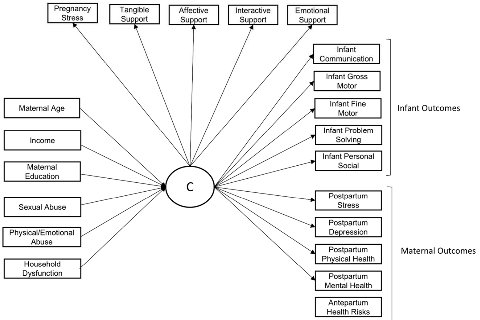
Supplementary Figure 1. Conceptual model tested for the latent profile analysis. C= latent class grouping.
