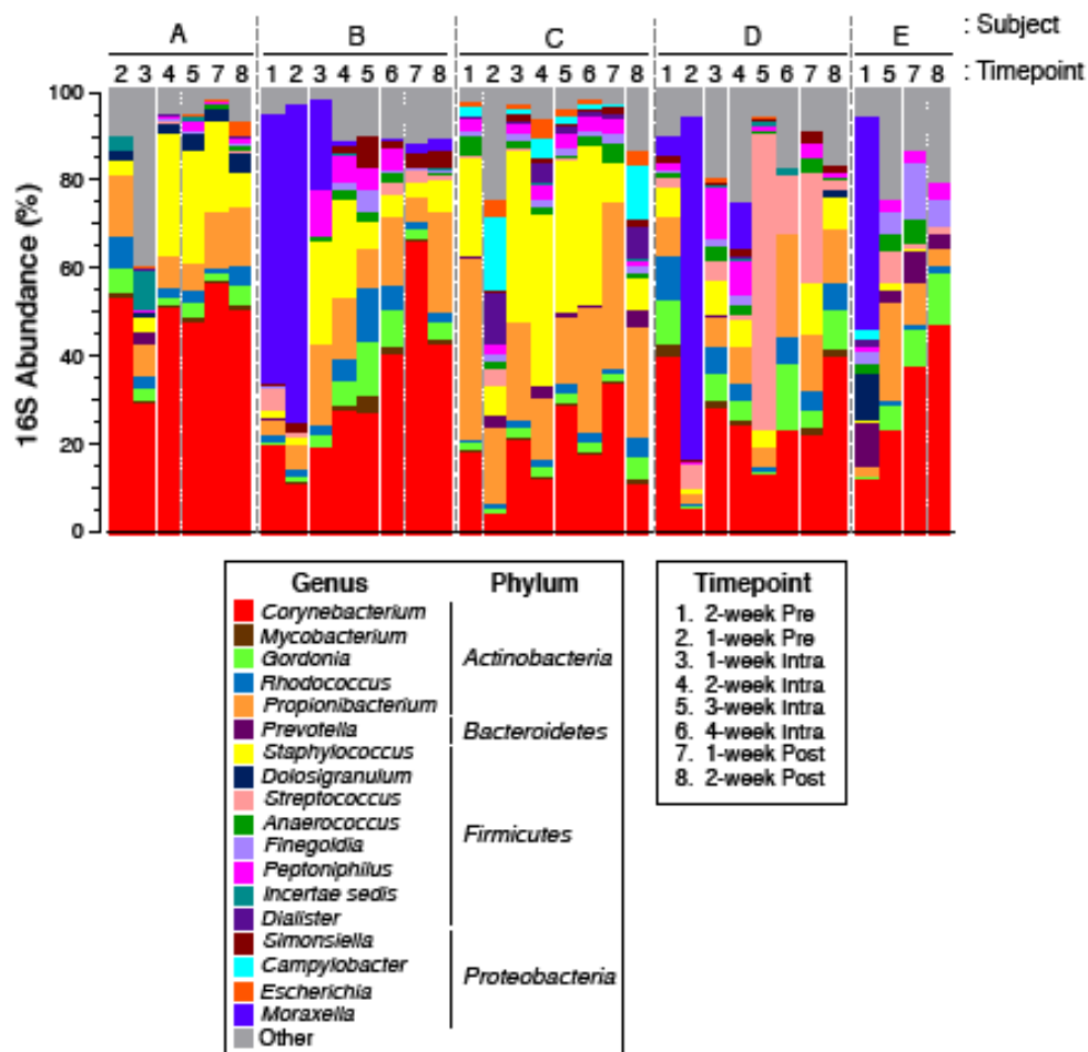
Supplemental Figure 1. Changes in nasal microbiota accompanying INS and mupirocin treatment. Relative abundances of nasal bacterial genera (genera with mean relative abundances <0.5% are aggregated in the “Other” category) are displayed for each sampling timepoint (1 week intervals). The legend displays the color-coding of genera, along with the phyla to which these taxa belong (i.e., Actinobacteria, Bacteroidetes, Firmicutes, Proteobacteria). Subjects A-D were treated with intranasal steroids while subject E was treated with topical mupirocin.
